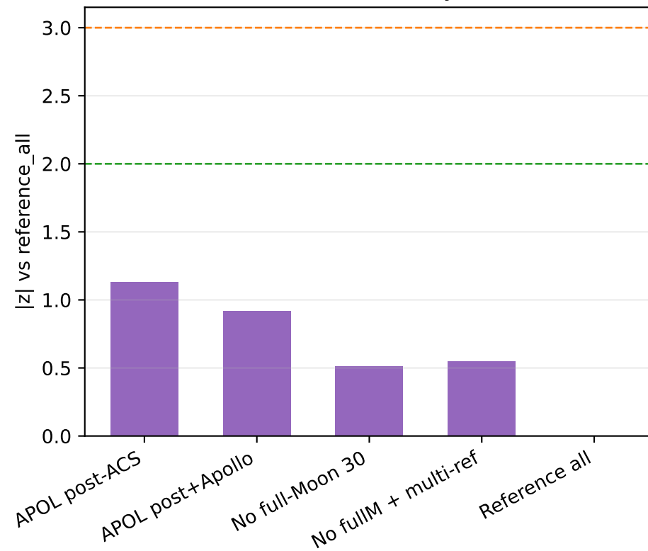
Subset stability
