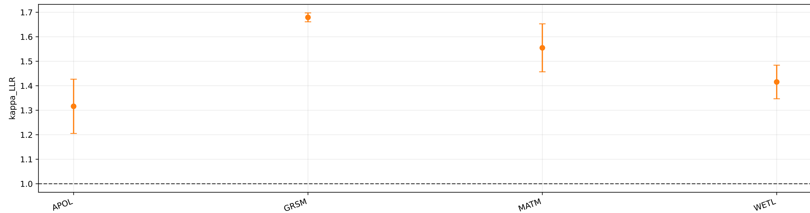
Station-stratified refit
