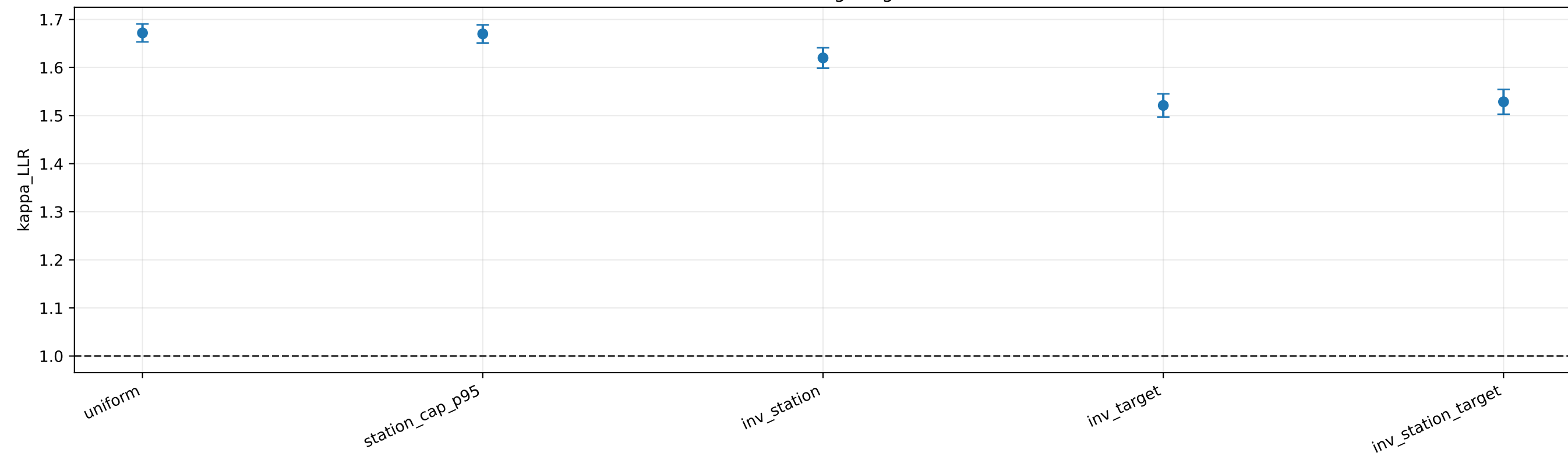
Station-stratified refit
