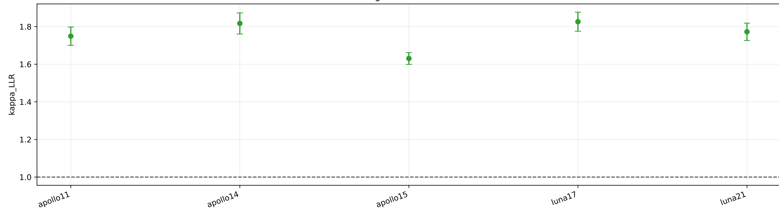
Target-stratified refit
