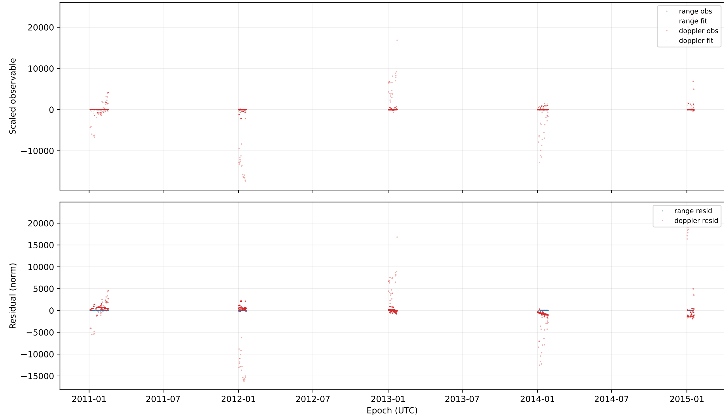
Roadmap 8.7.48.4: Stage D joint fit (range + doppler)
