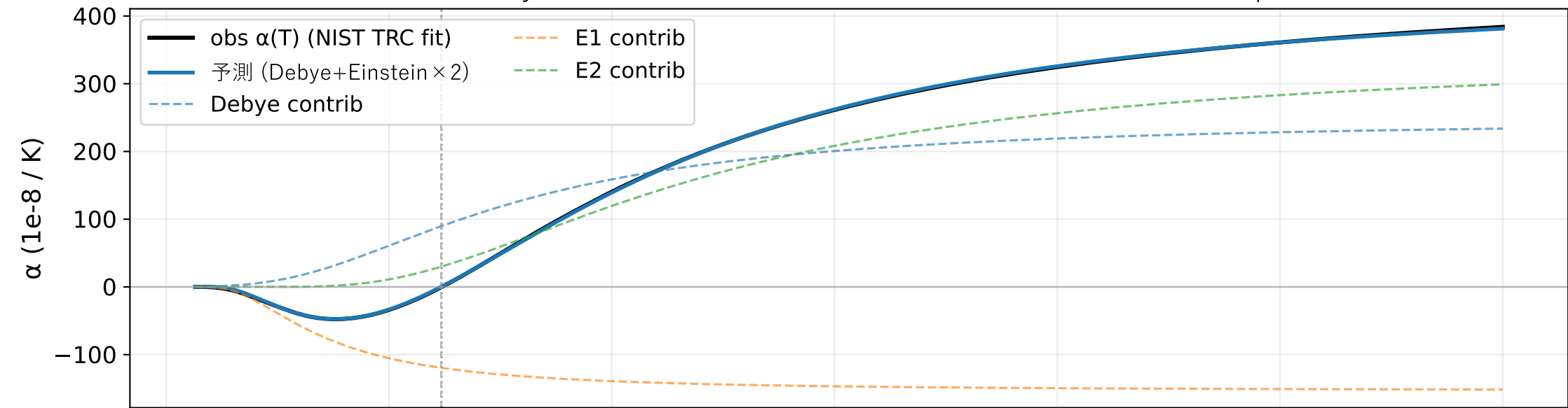
Si 熱膨張: Debye+Einstein \times 2 with \theta_E anchors from Ioffe フォノン frequencies
