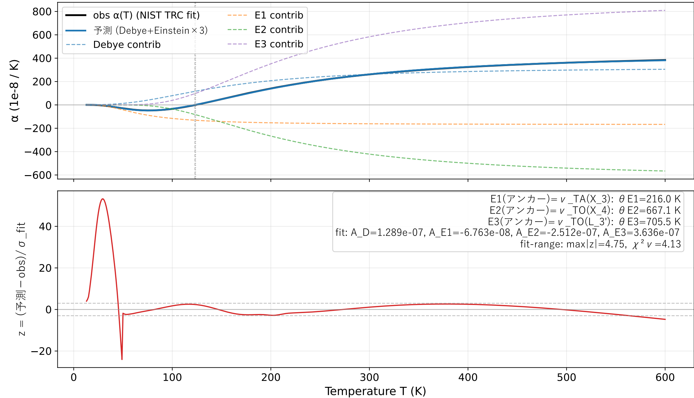
Si 熱膨張: Debye+Einstein \times 3 with \theta_E anchors from Ioffe フォノン frequencies
