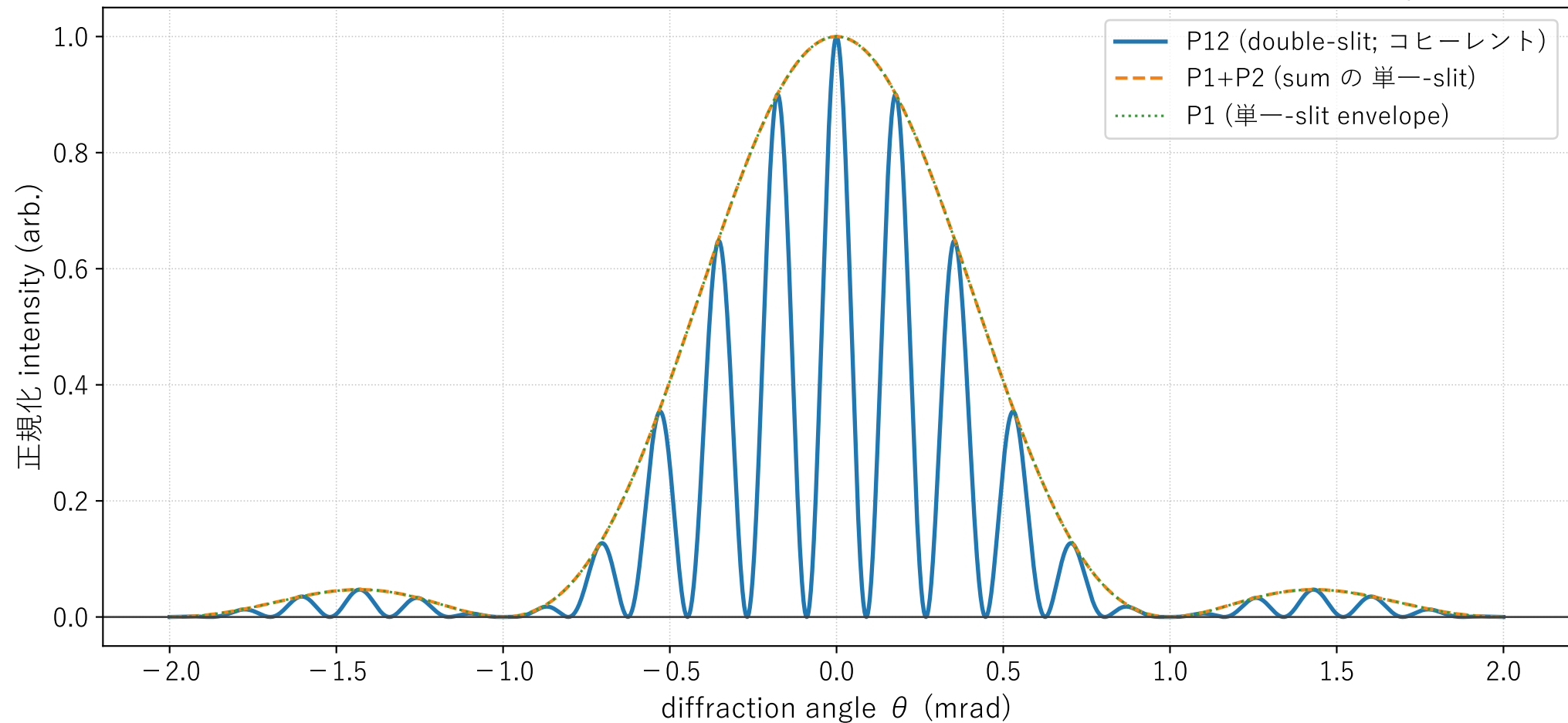
Electron double-slit diffraction (arXiv:1210.6243v1; 600 eV; 50 nm slits, 280 nm sep.)
