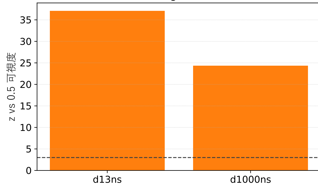
HOM significance
