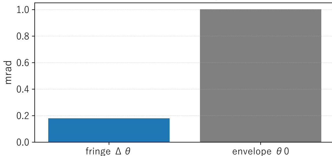
Electron double-slit angular scales
