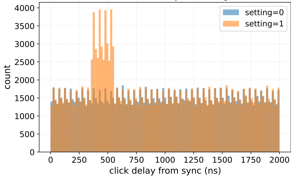
Alice: click delay vs setting
