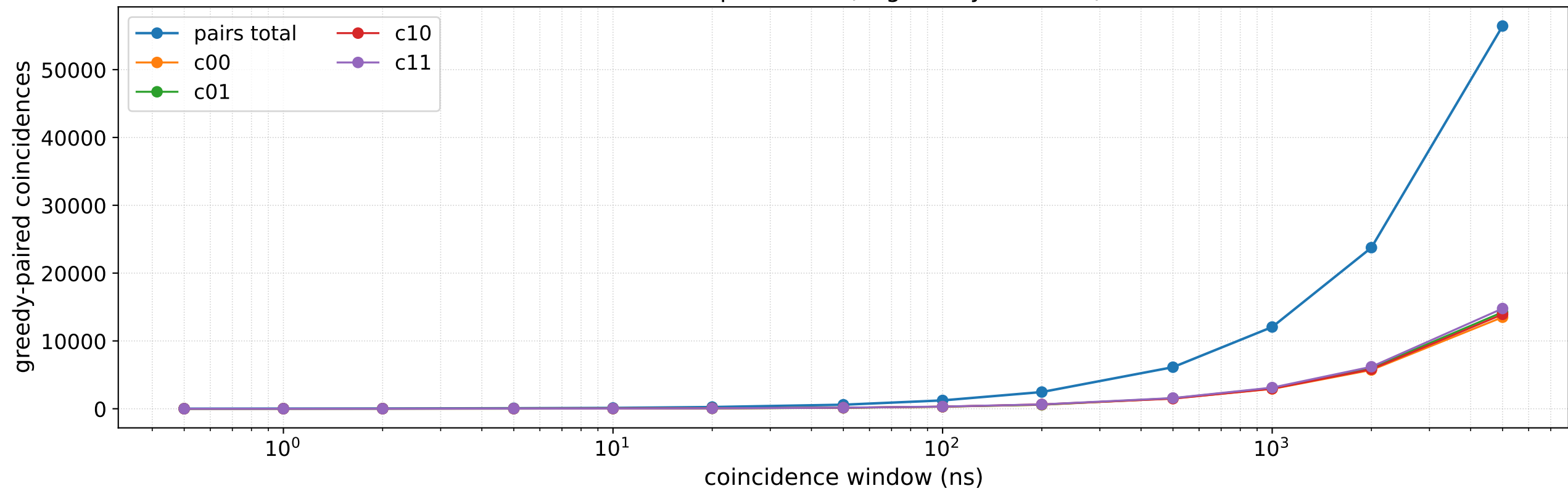
Window dependence (aligned by GPS PPS)
