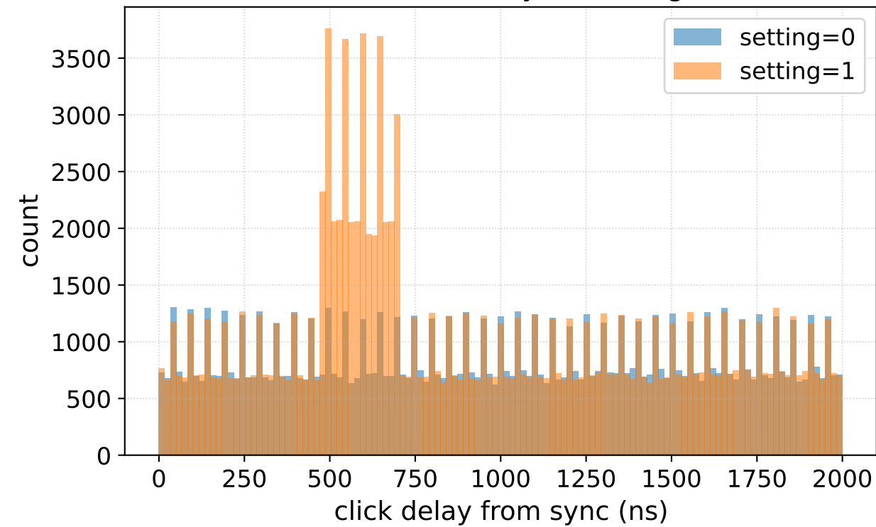
Bob: click delay vs setting
