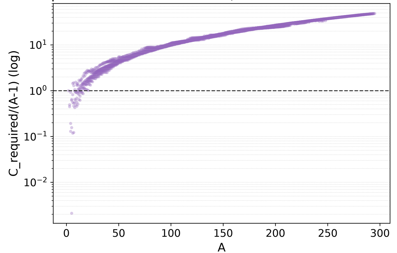
Implied coherence factor vs A (needs >1 for extra binding)
