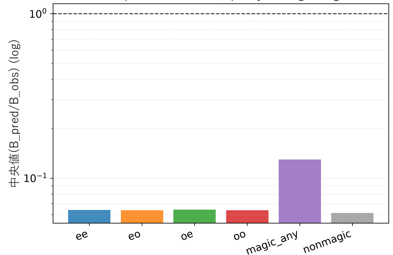
Group medians (基準): parity & magic flags
