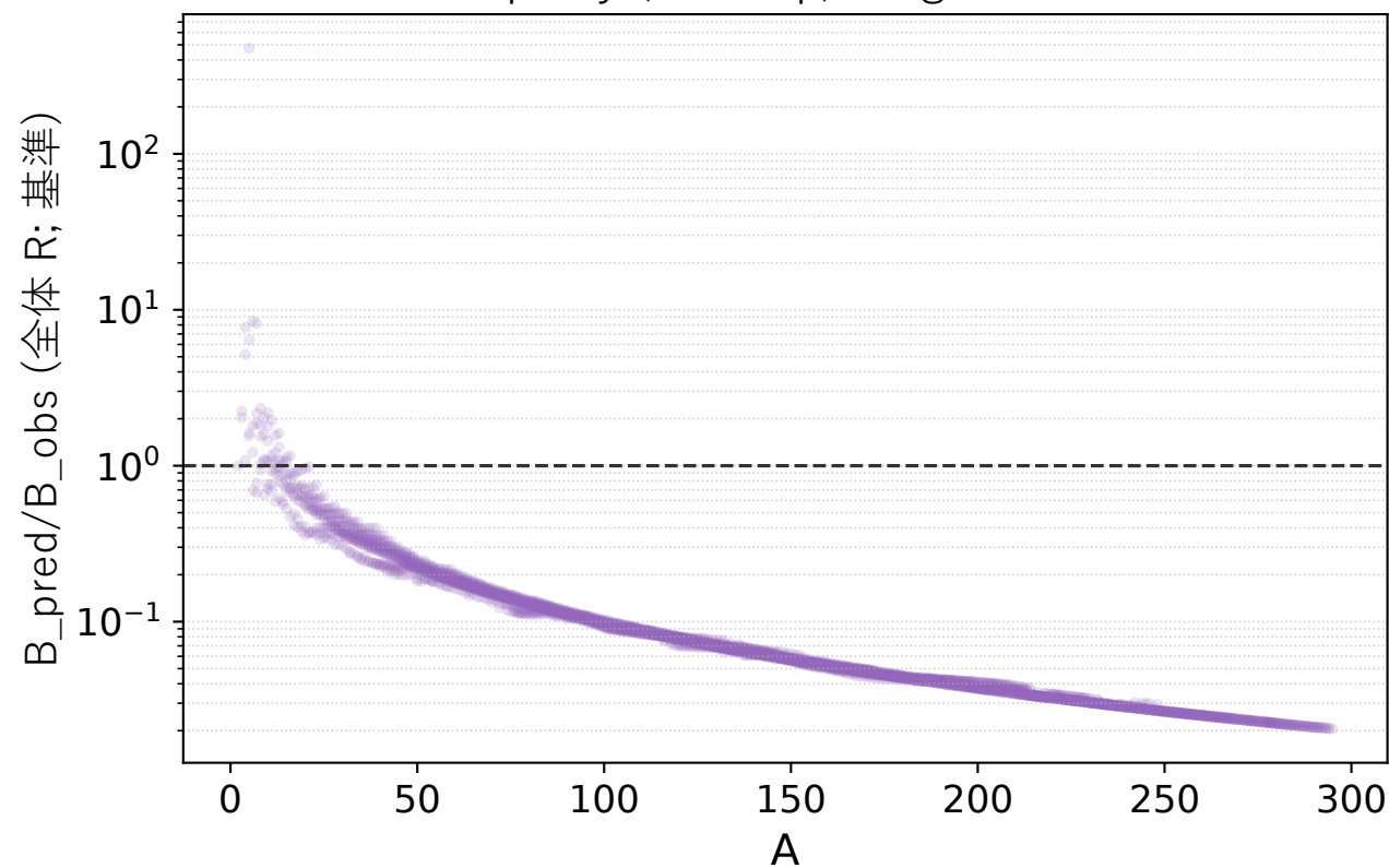
全体 distance proxy (R in exp): large A-trend mismatch
