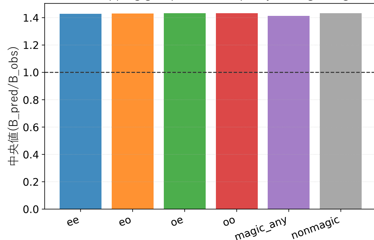
局所 mapping group medians (parity & magic flags)
