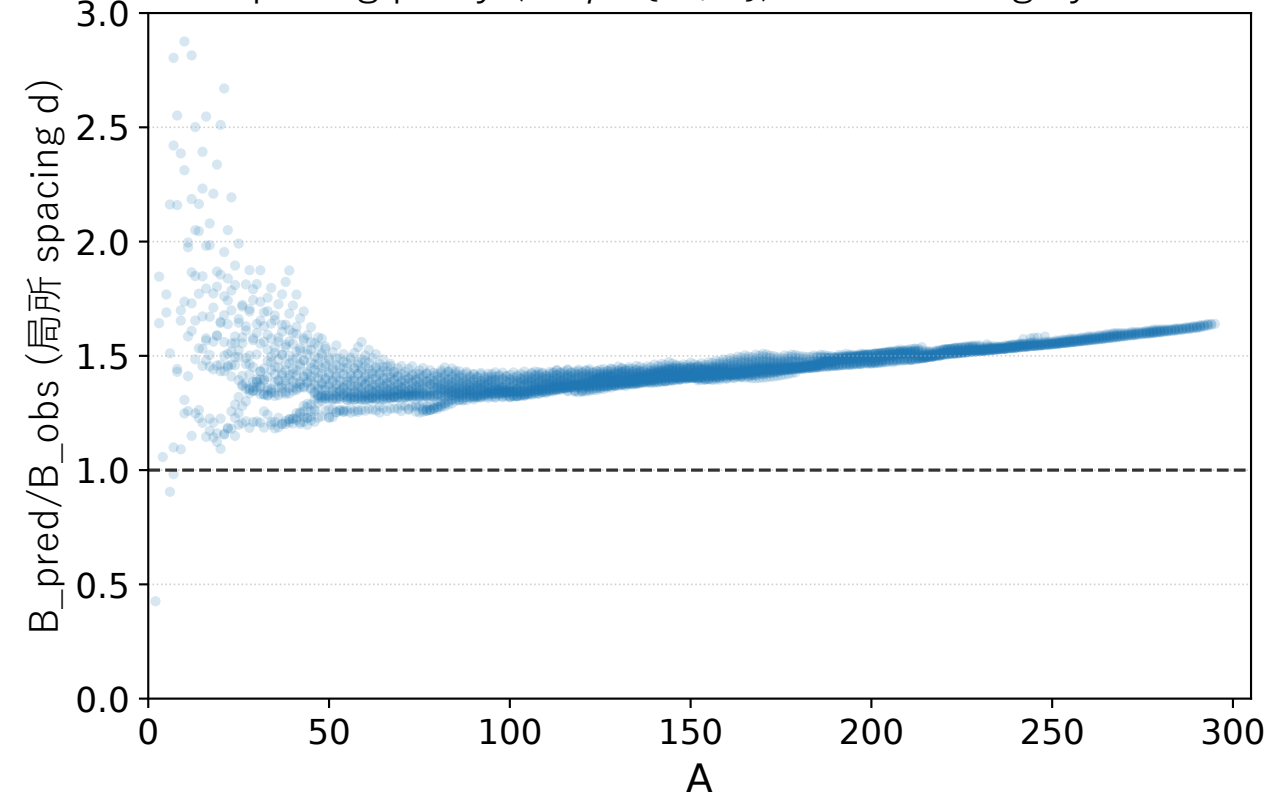
局所 spacing proxy ( d = \rho^{-1/3} ): A-trend largely removed
