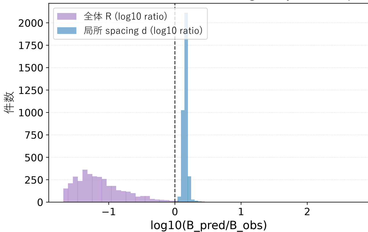
残差 distributions (same frozen アンカー/range; only distance proxy differs)
