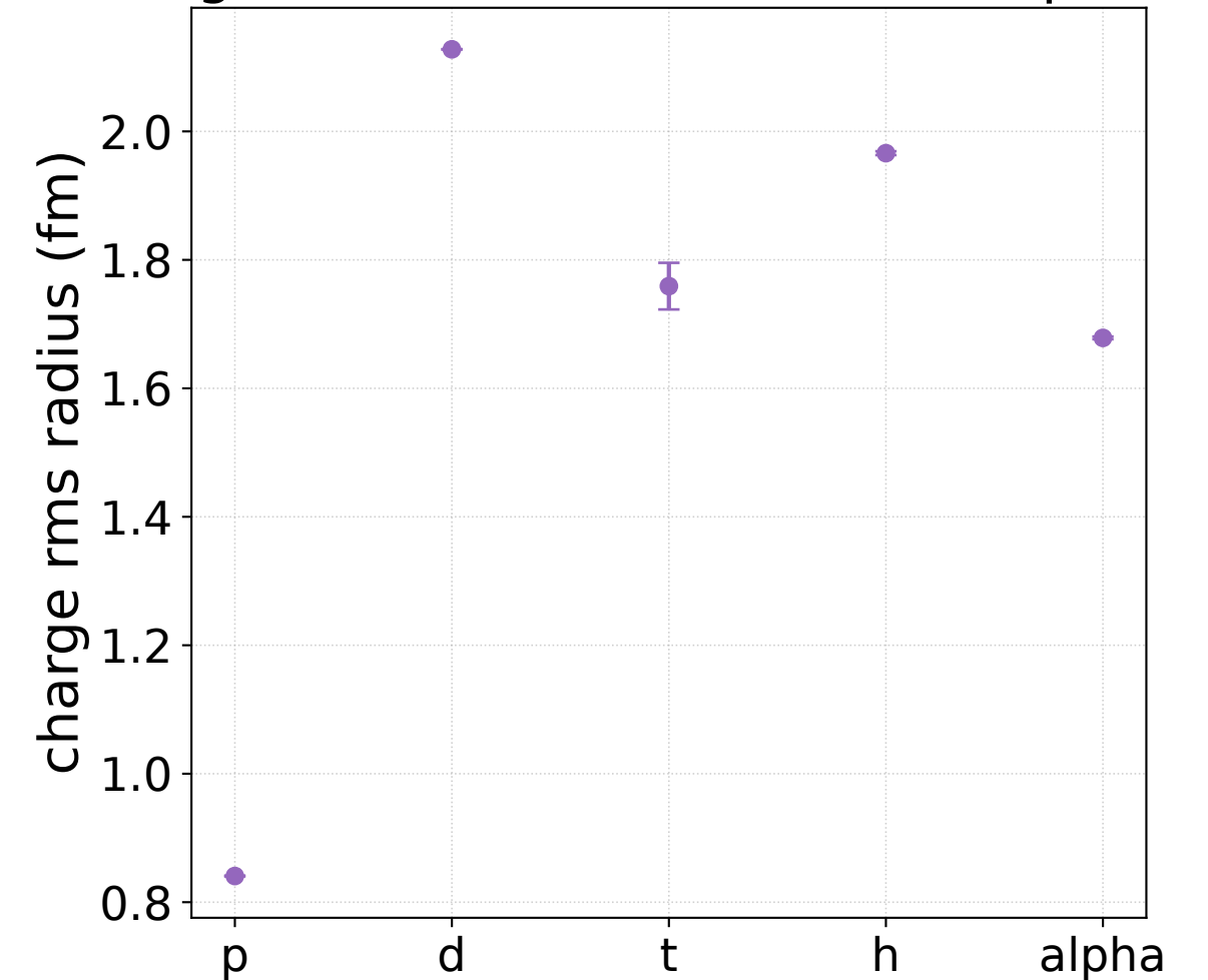
Charge radii (CODATA + IAEA compilation)
