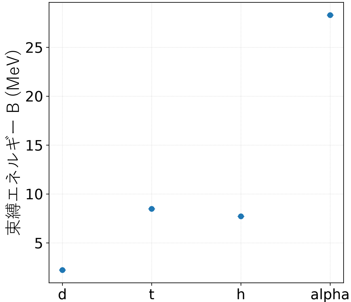
Mass defect 基準 (CODATA via NIST)
