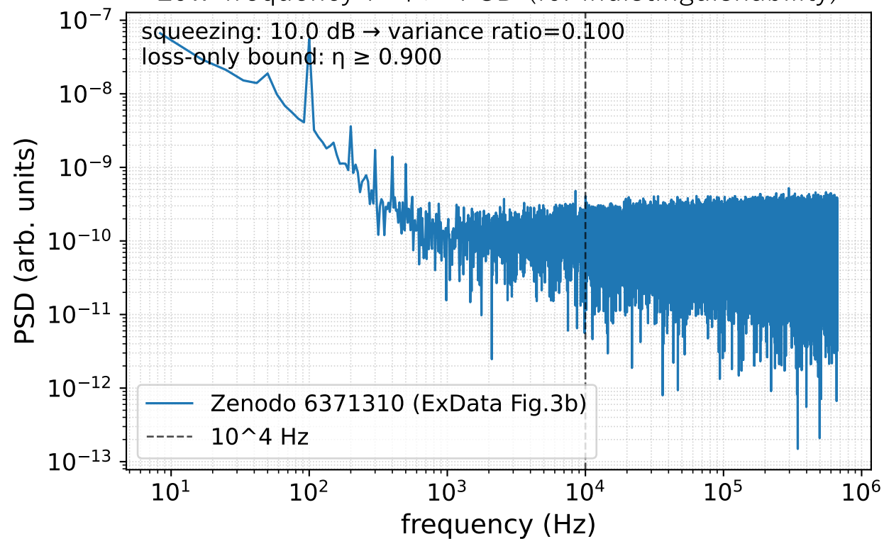
Low-frequency ノイズ PSD (for indistinguishability)
