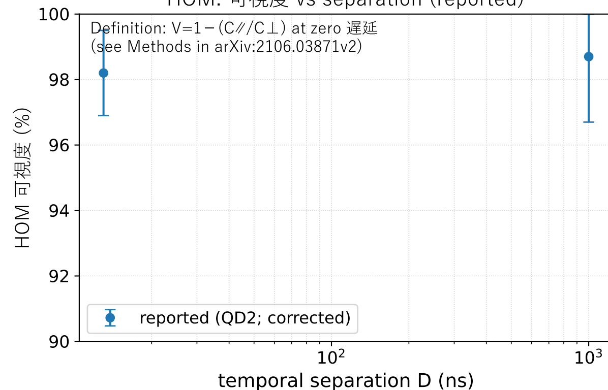
HOM: 可視度 vs separation (reported)
