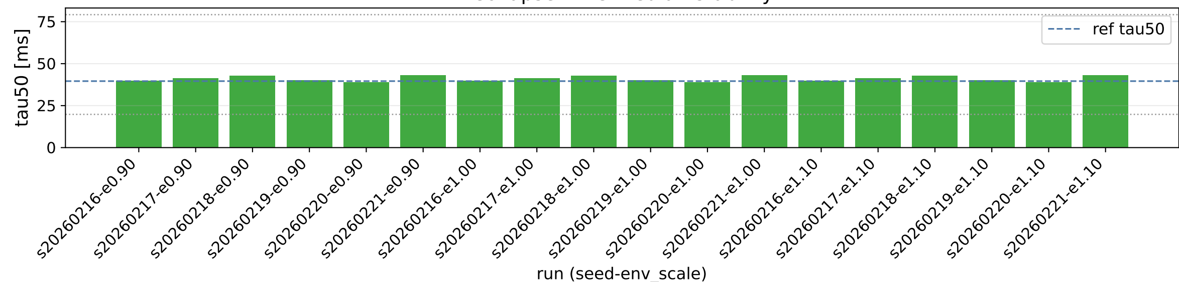
Branch-stability gate
