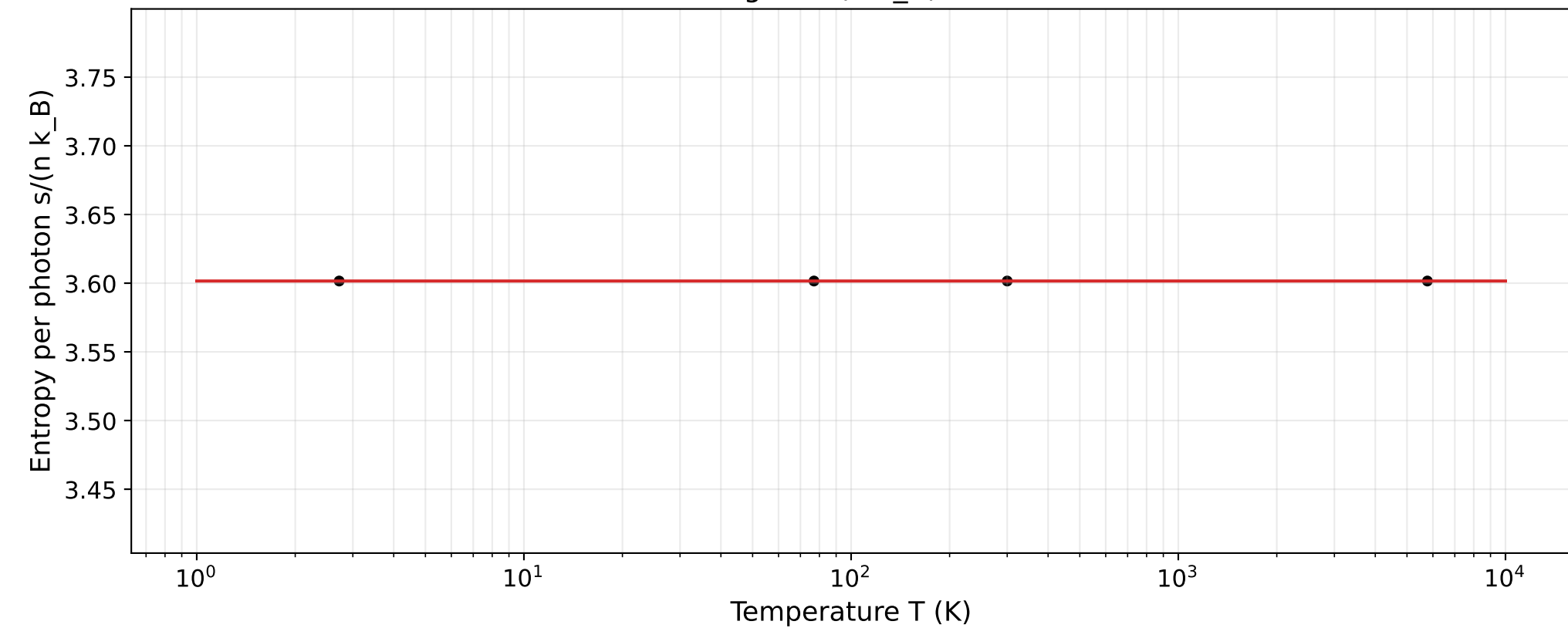
Photon gas: s/(n k_B) = \text{const.}
