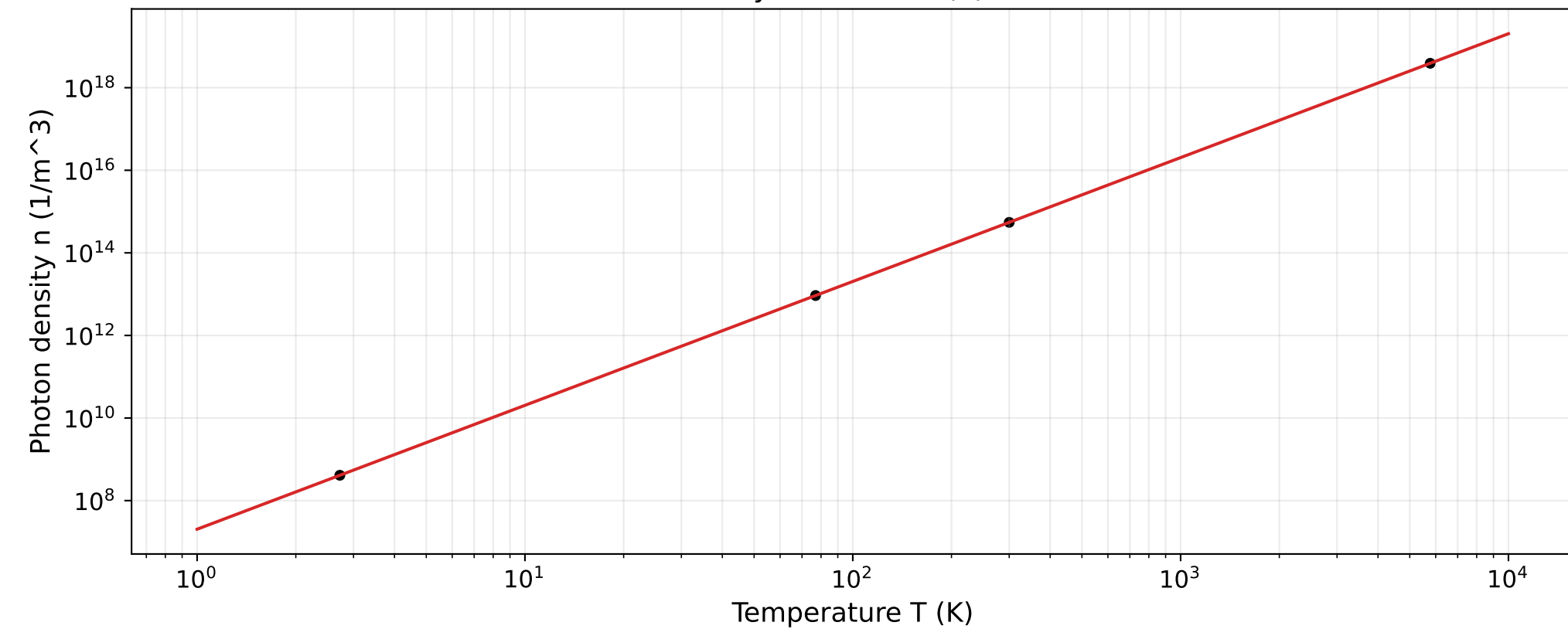
Blackbody radiation: n(T) \propto T^3
