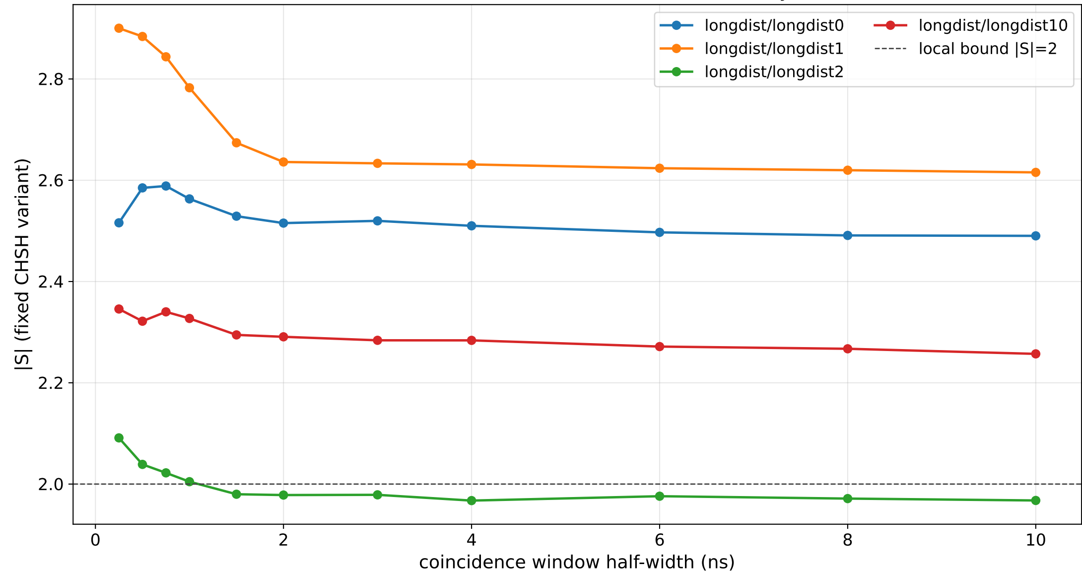
Weihs 1998 (Zenodo 7185335): coincidence-window sensitivity across runs/subdirs
