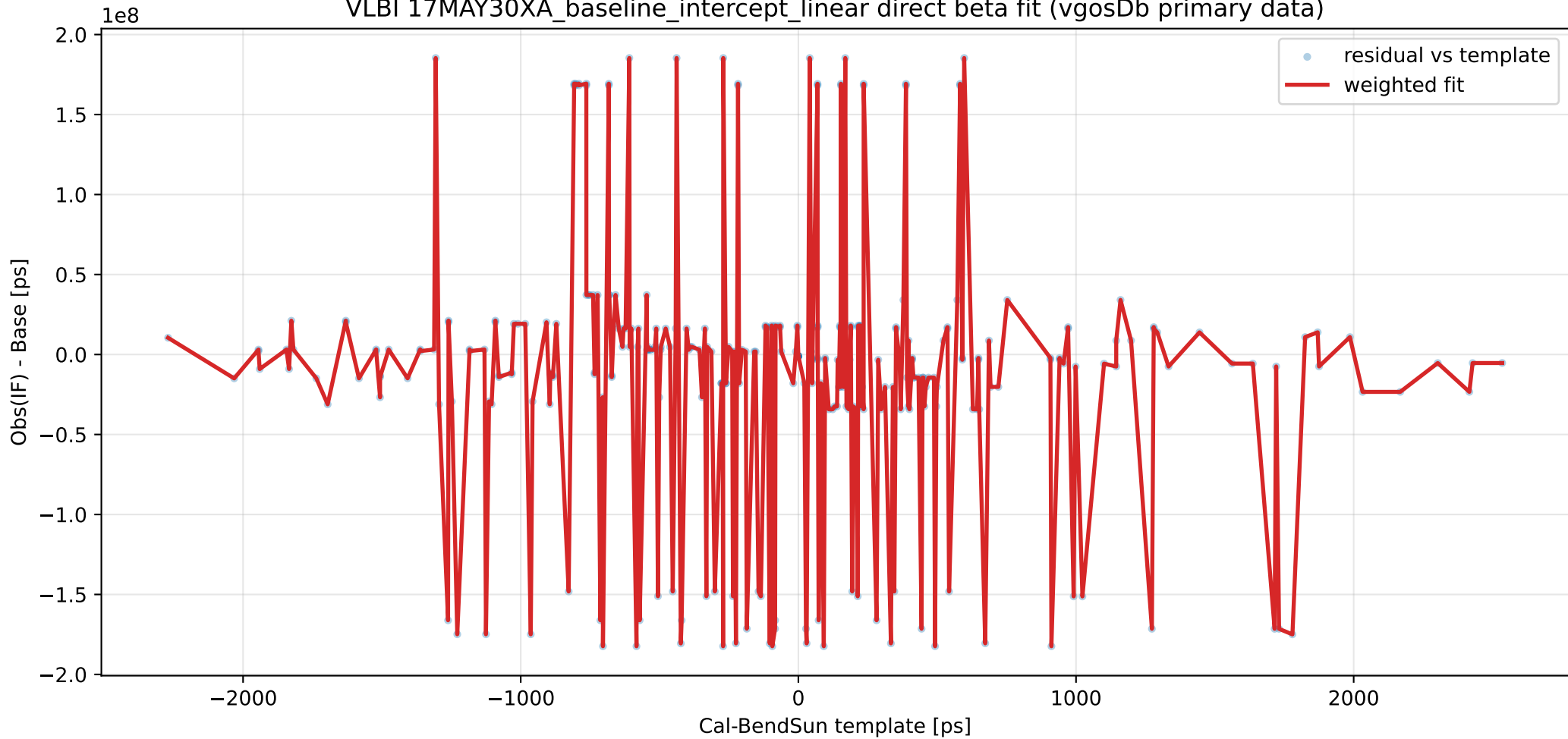
VLBI 17MAY30XA_baseline_intercept_linear direct beta fit (vgosDb primary data)
