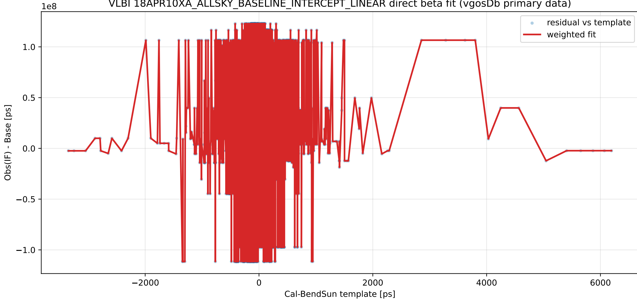
VLBI 18APR10XA_ALLSKY_BASELINE_INTERCEPT_LINEAR direct beta fit (vgosDb primary data)
