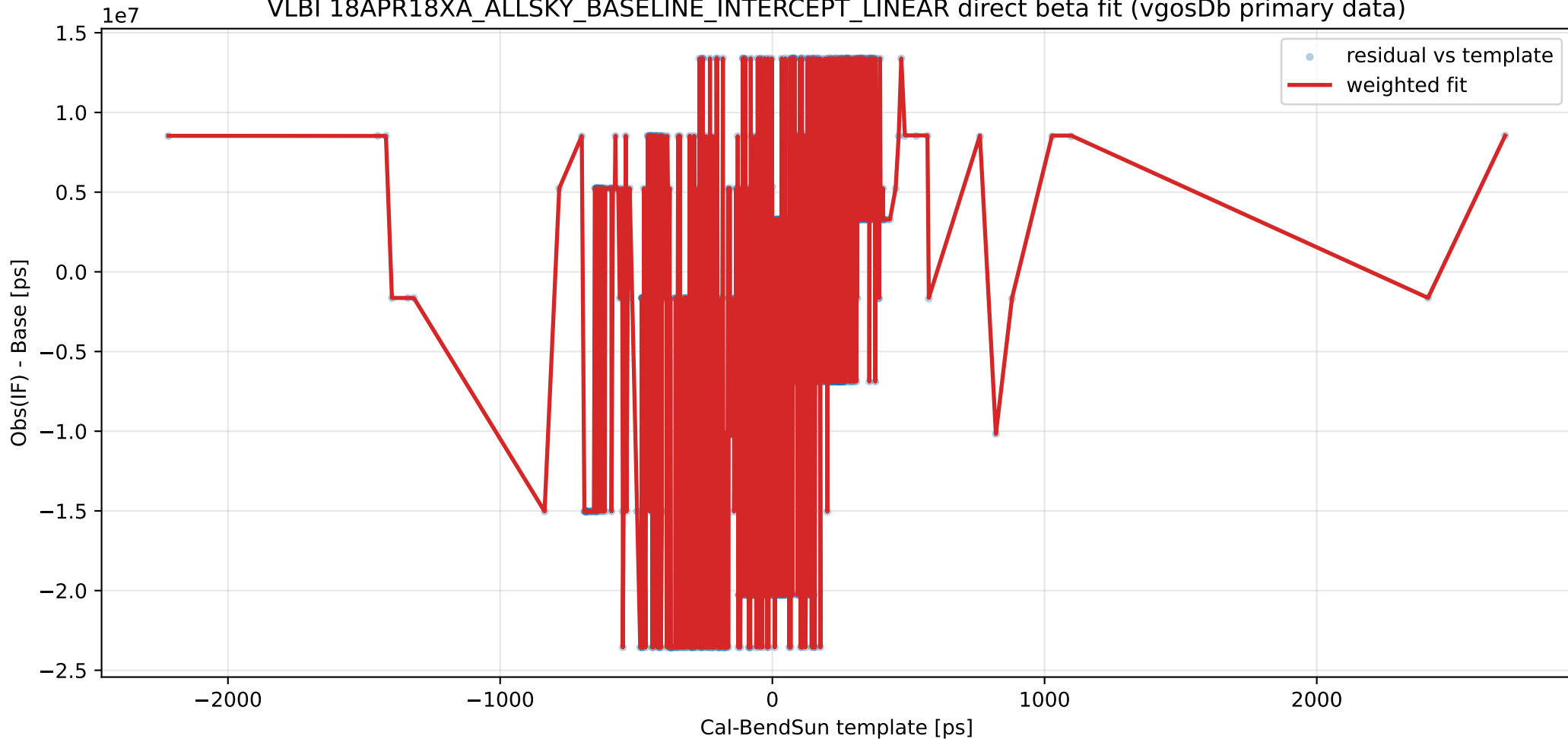
VLBI 18APR18XA_ALLSKY_BASELINE_INTERCEPT_LINEAR direct beta fit (vgosDb primary data)
