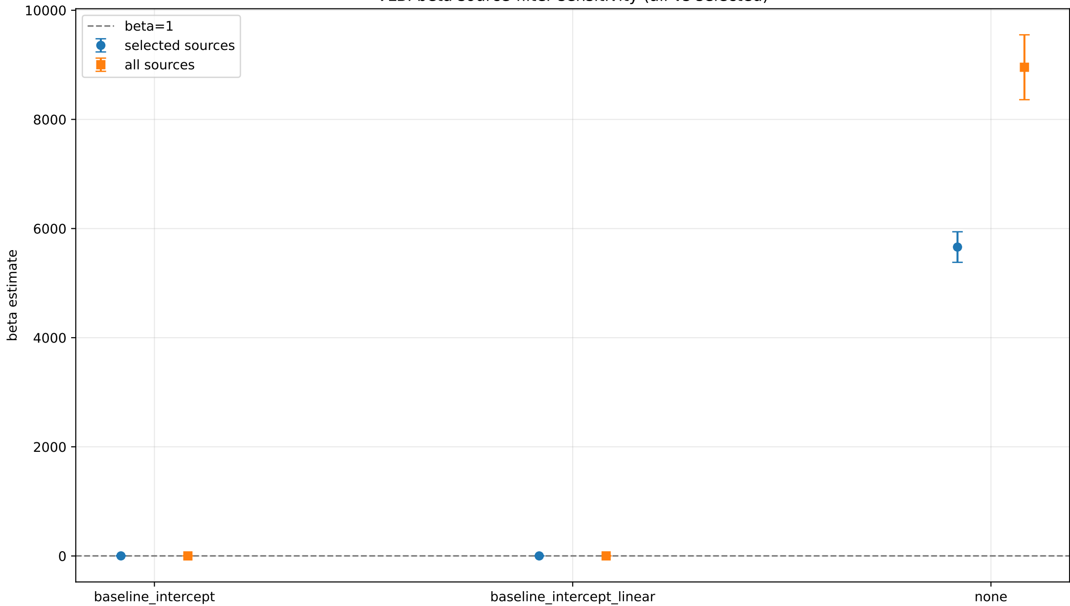
VLBI beta source-filter sensitivity (all vs selected)
