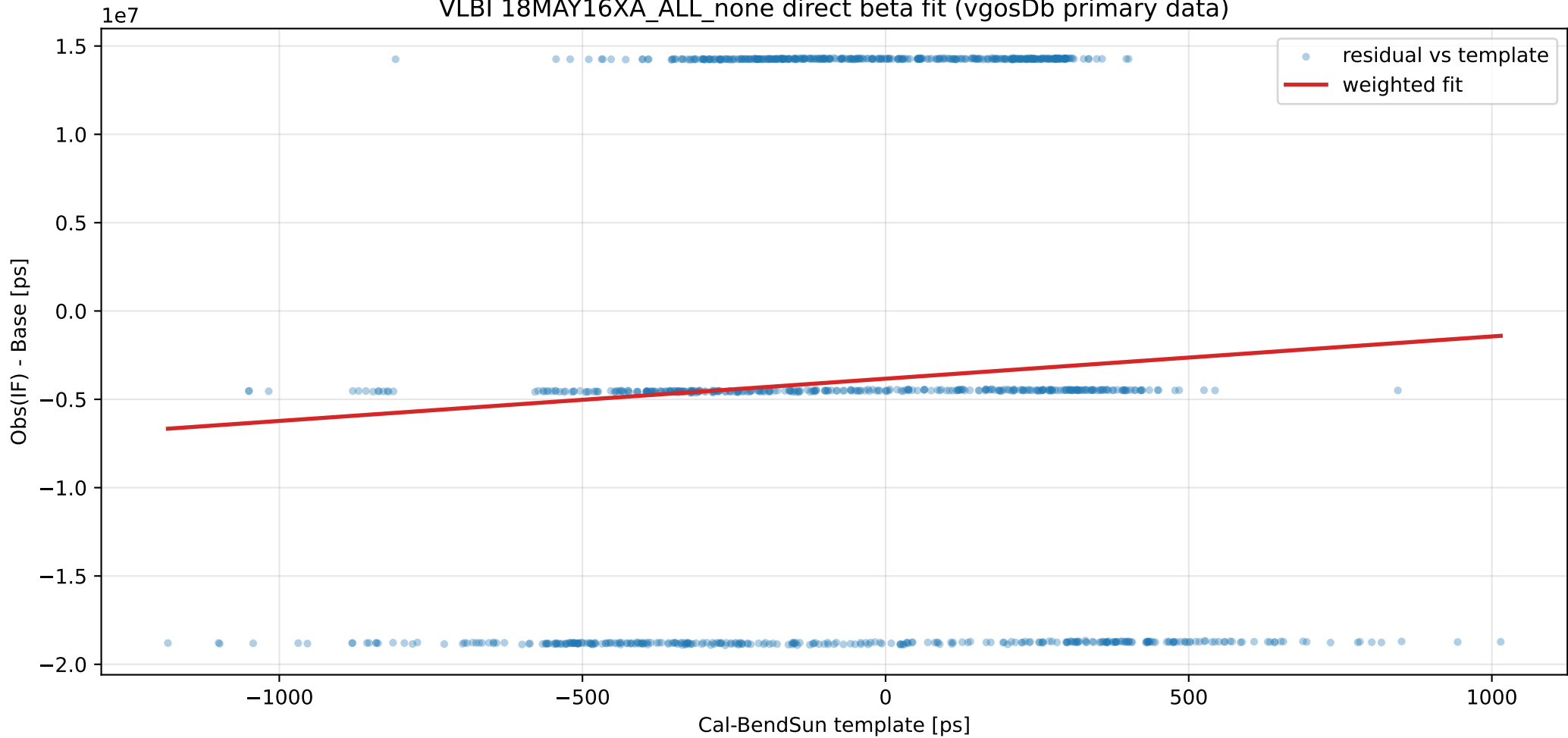
VLBI 18MAY16XA_ALL_none direct beta fit (vgosDb primary data)
