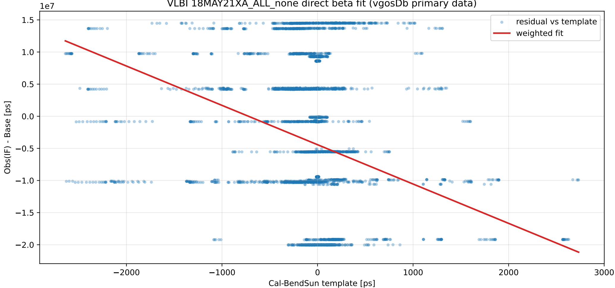
VLBI 18MAY21XA_ALL_none direct beta fit (vgosDb primary data)
