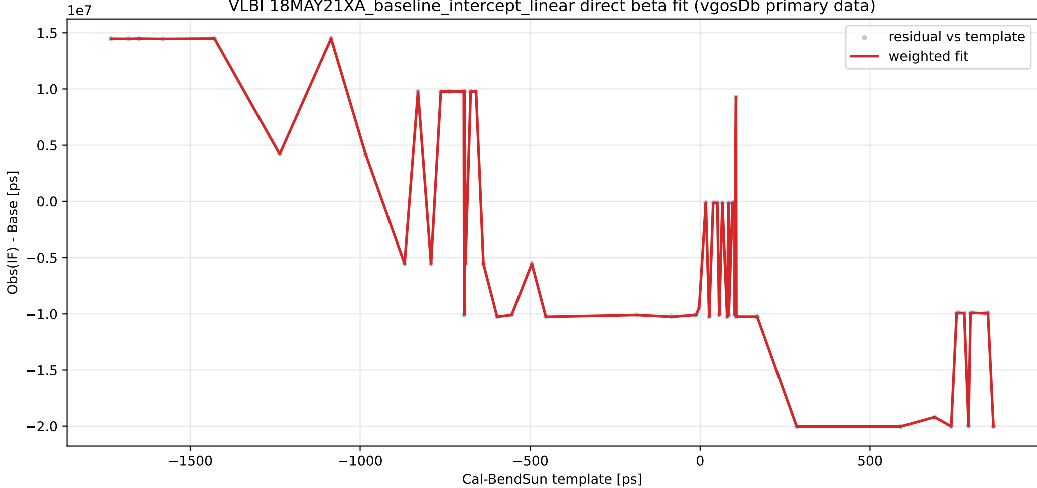
VLBI 18MAY21XA_baseline_intercept_linear direct beta fit (vgosDb primary data)
