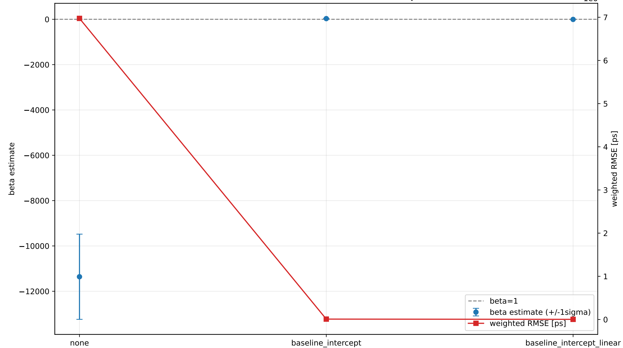
VLBI beta direct-fit nuisance sensitivity
