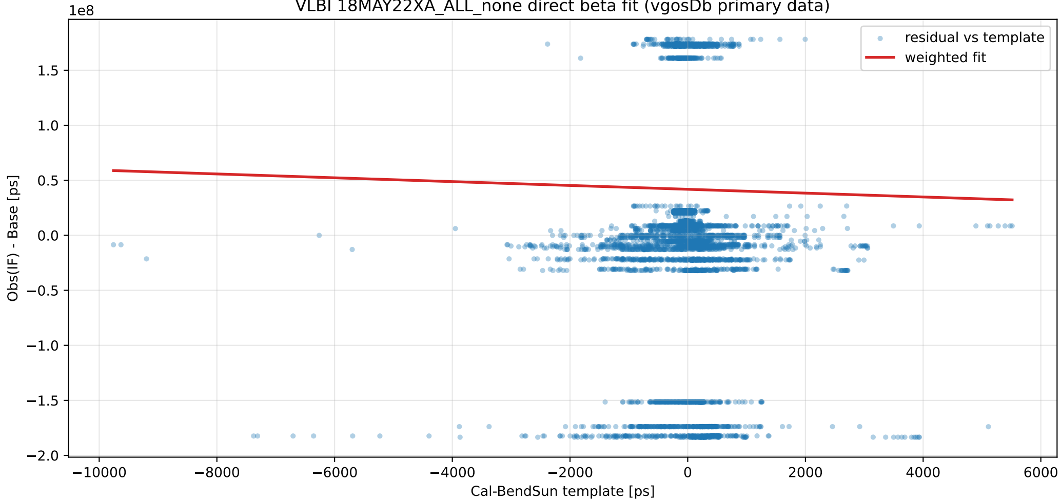
VLBI 18MAY22XA_ALL_none direct beta fit (vgosDb primary data)
