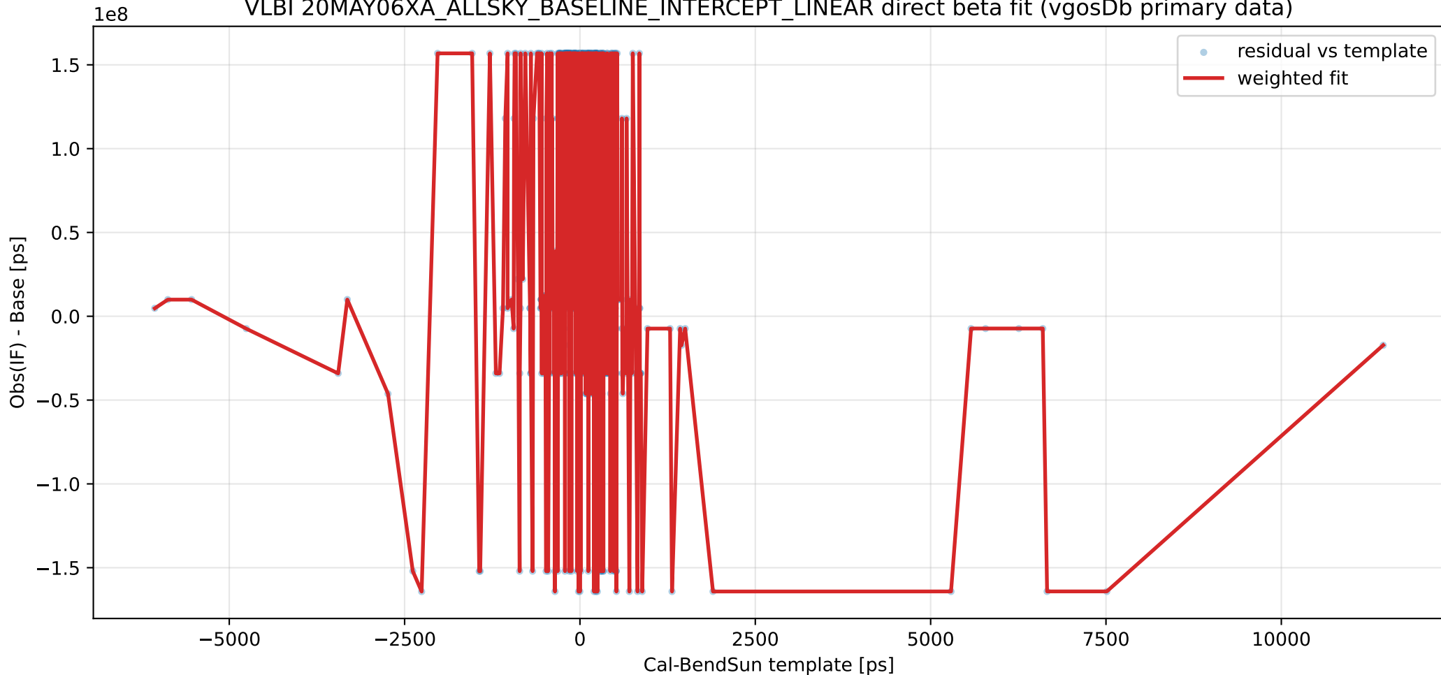
VLBI 20MAY06XA_ALLSKY_BASELINE_INTERCEPT_LINEAR direct beta fit (vgosDb primary data)
