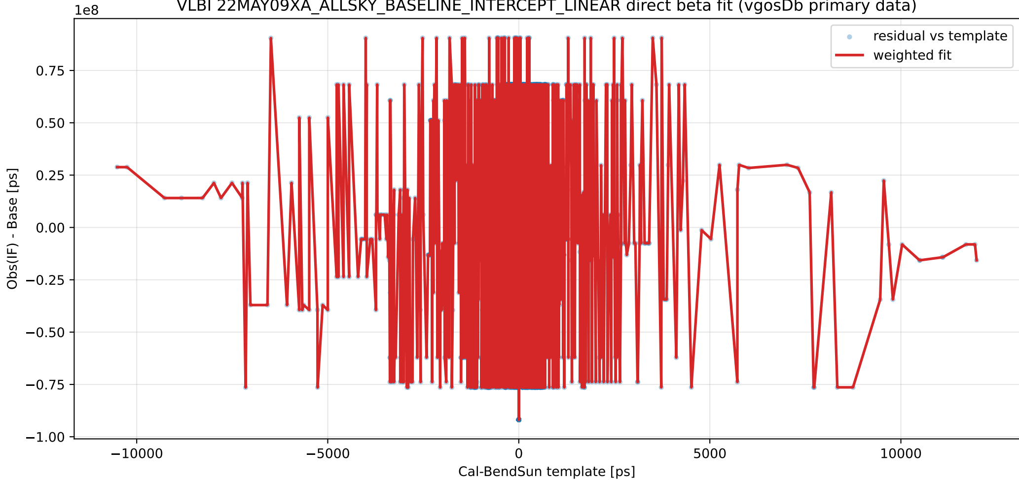
VLBI 22MAY09XA_ALLSKY_BASELINE_INTERCEPT_LINEAR direct beta fit (vgosDb primary data)
