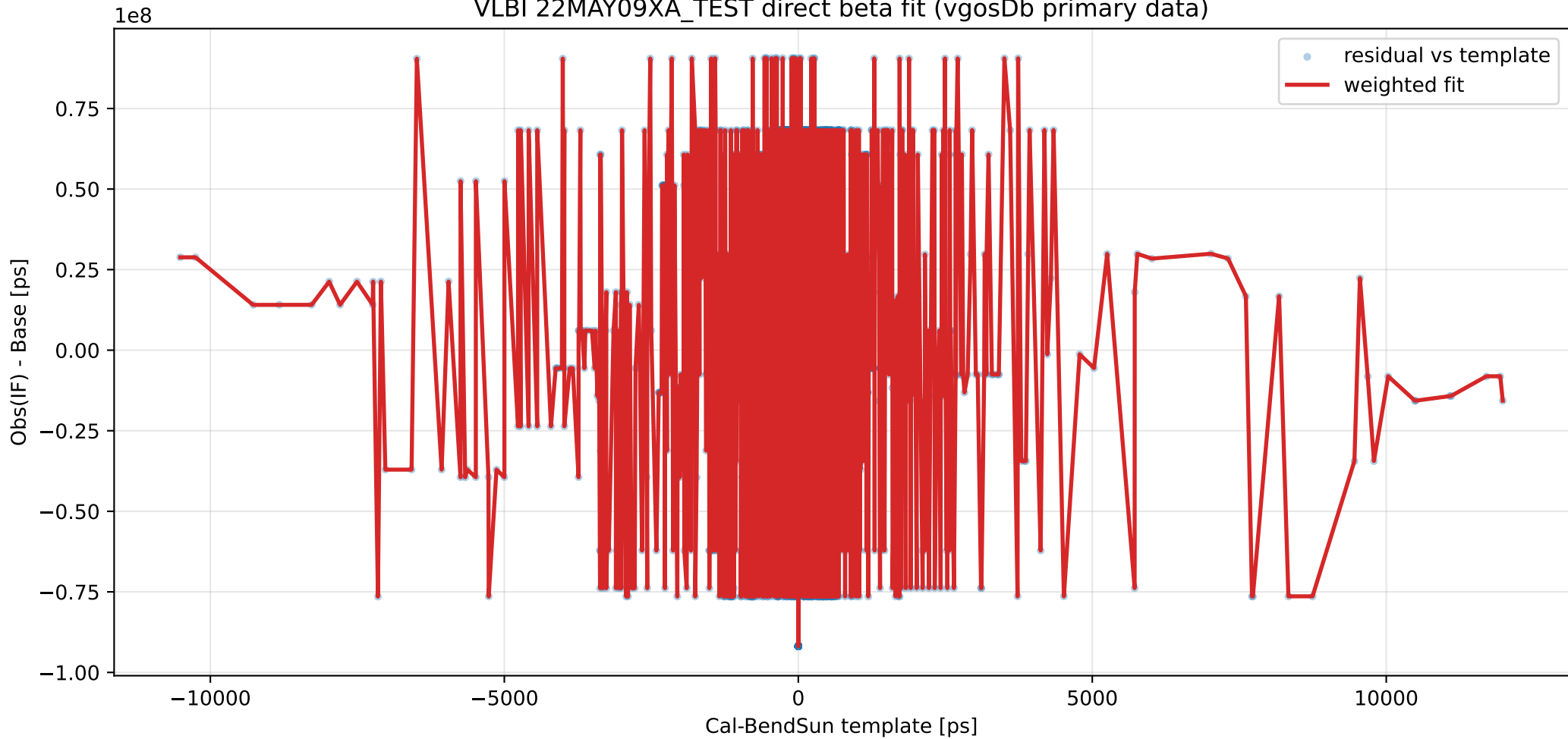
VLBI 22MAY09XA_TEST direct beta fit (vgosDb primary data)
