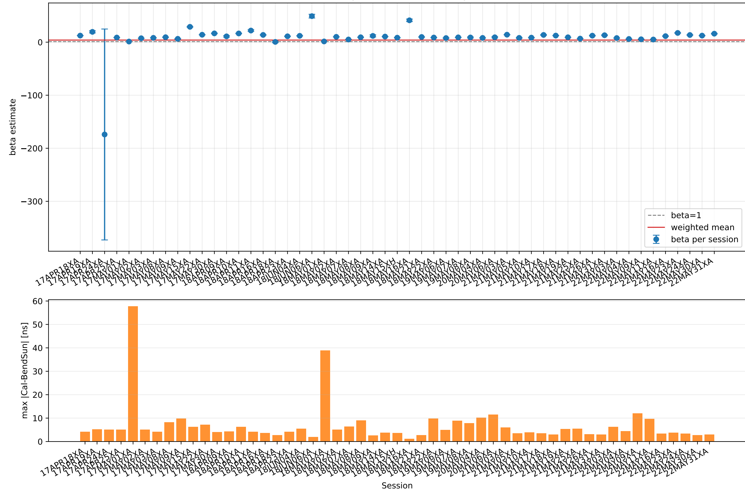
All-sky VLBI beta consistency
