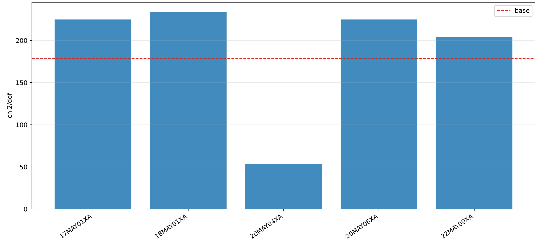
High-sensitivity leave-one-out consistency
