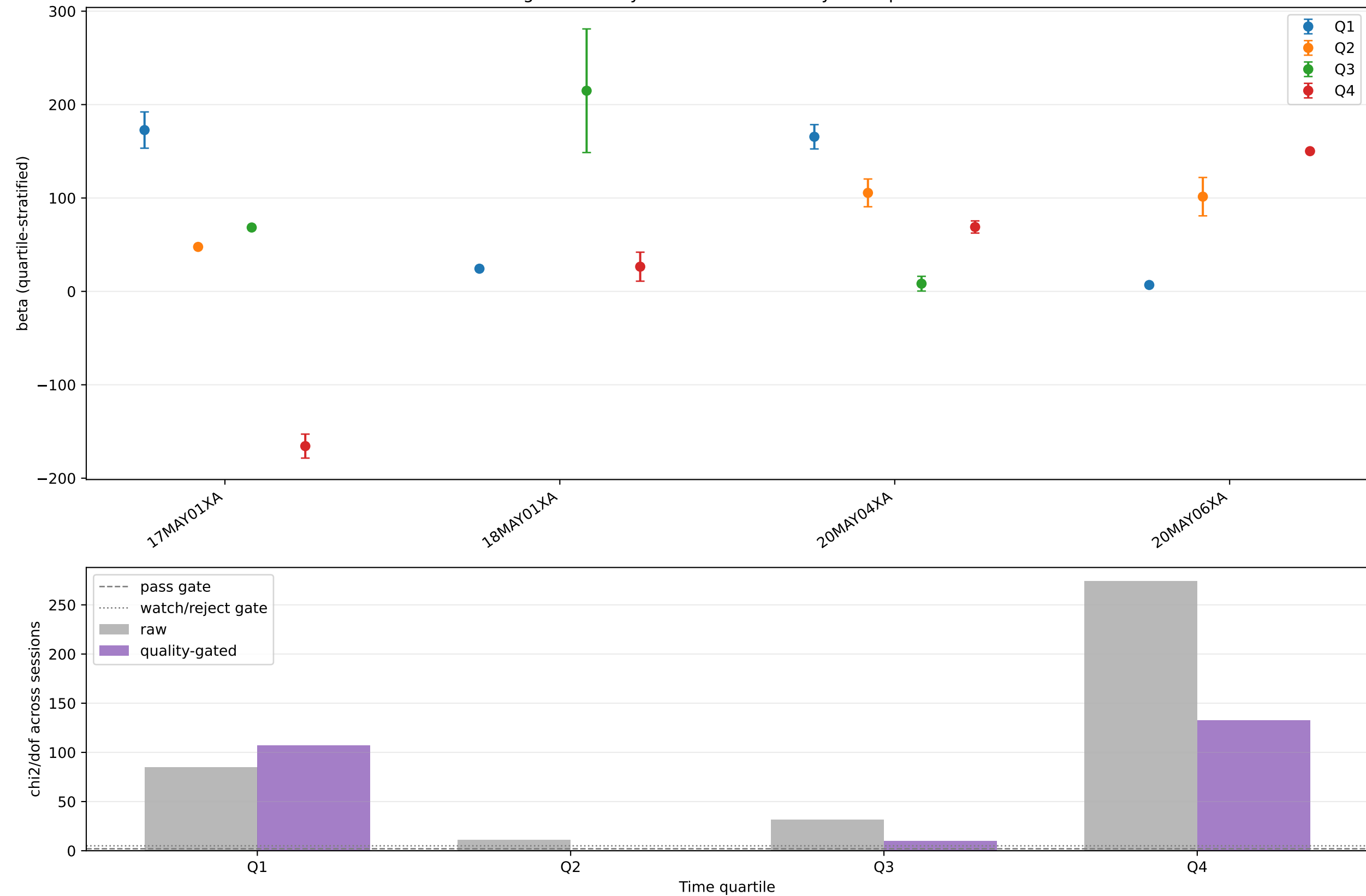
High-sensitivity stable-source refit by time quartile
