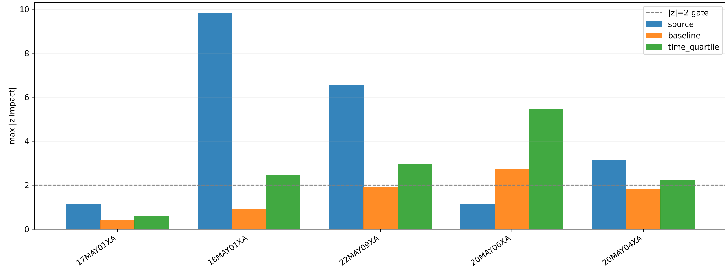
High-sensitivity VLBI factor decomposition (drop-one)
