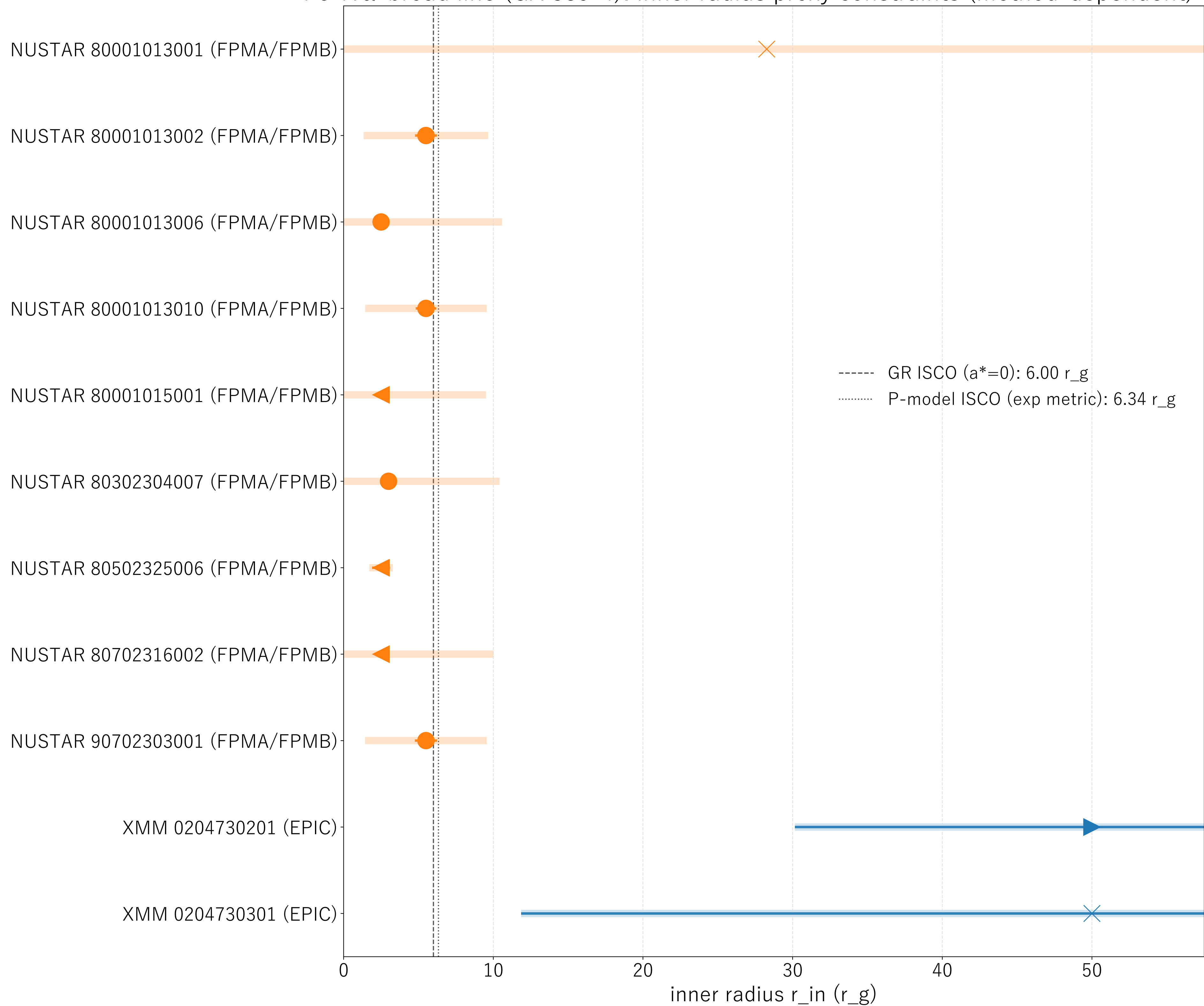
Fe-K \alpha broad line (GX 339-4): inner radius proxy constraints (method-dependent)
