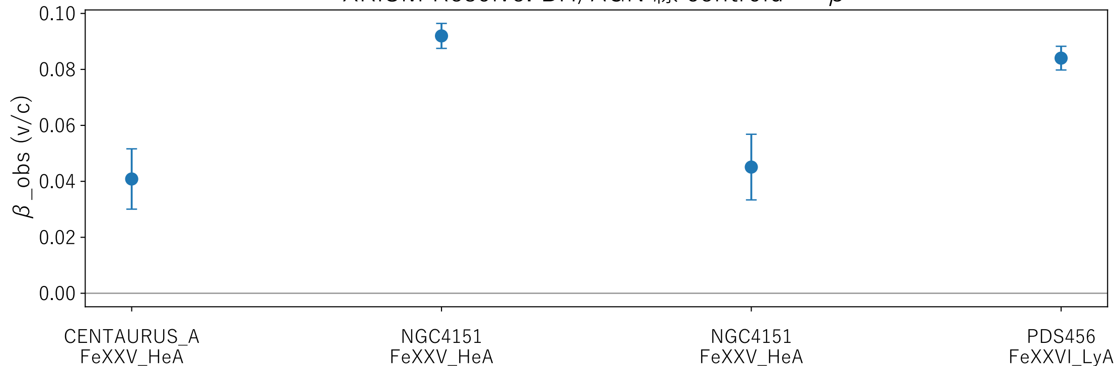
XRISM Resolve: BH/AGN 線 centroid \rightarrow \beta
