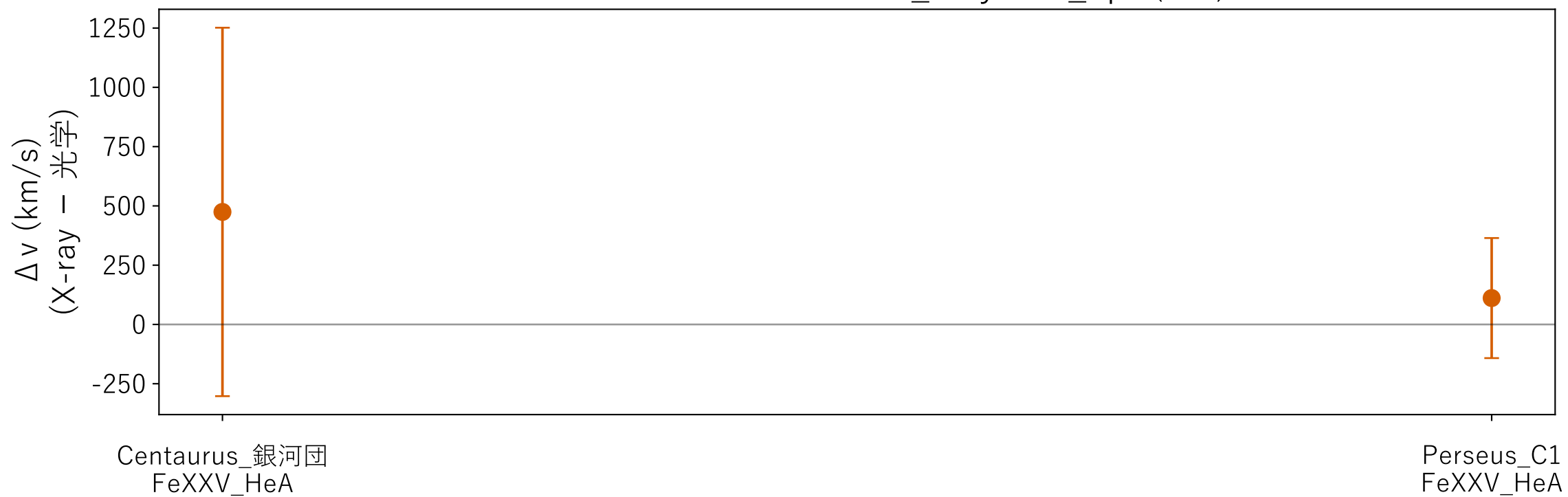
XRISM Resolve: clusters z_{\text{xray}} - z_{\text{opt}} (\Delta v)
