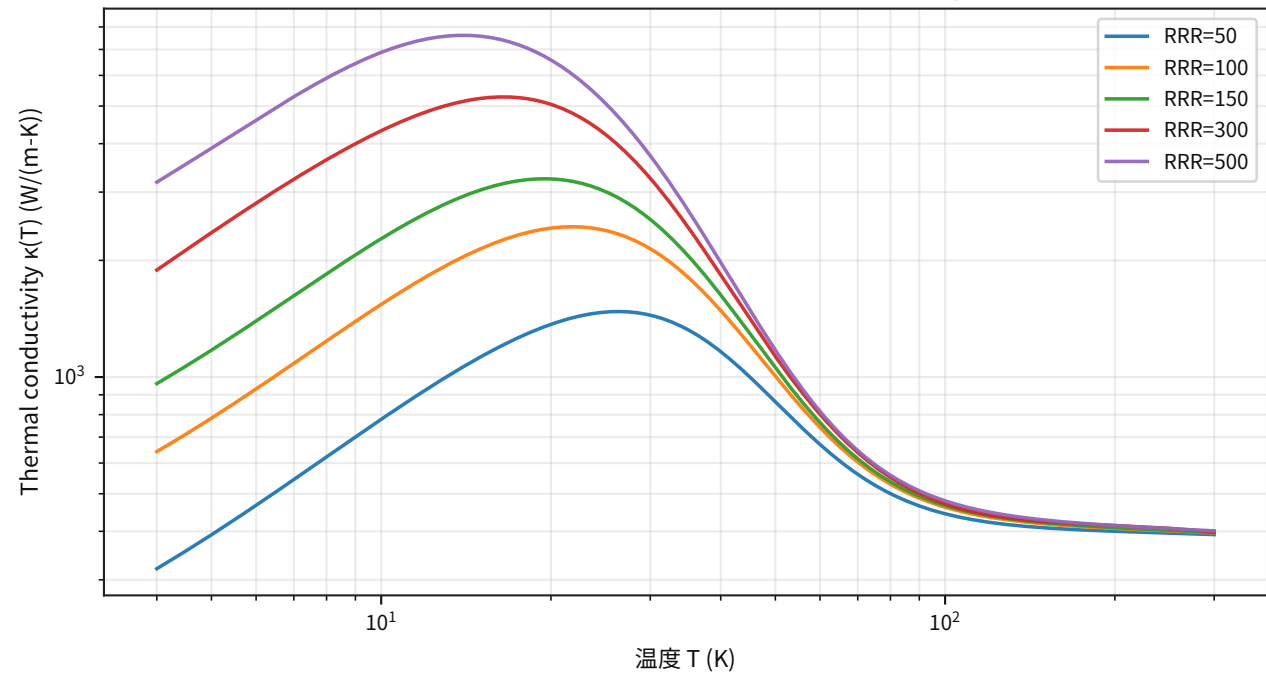
OFHC 銅 thermal conductivity \kappa(T) (NIST TRC cryogenics fit)
