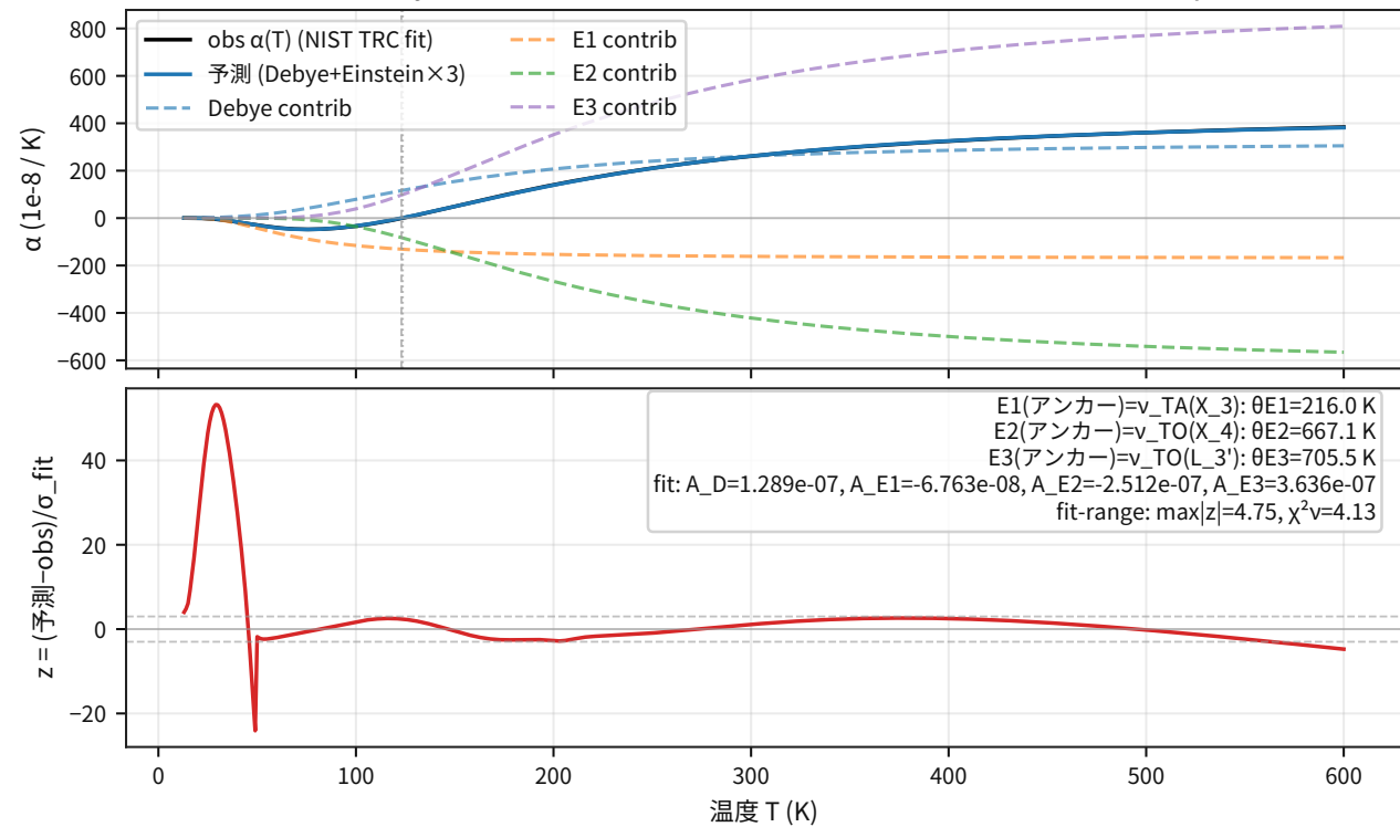
Si 熱膨張: Debye+Einstein×3 with \theta_E anchors from Ioffe フォノン frequencies
