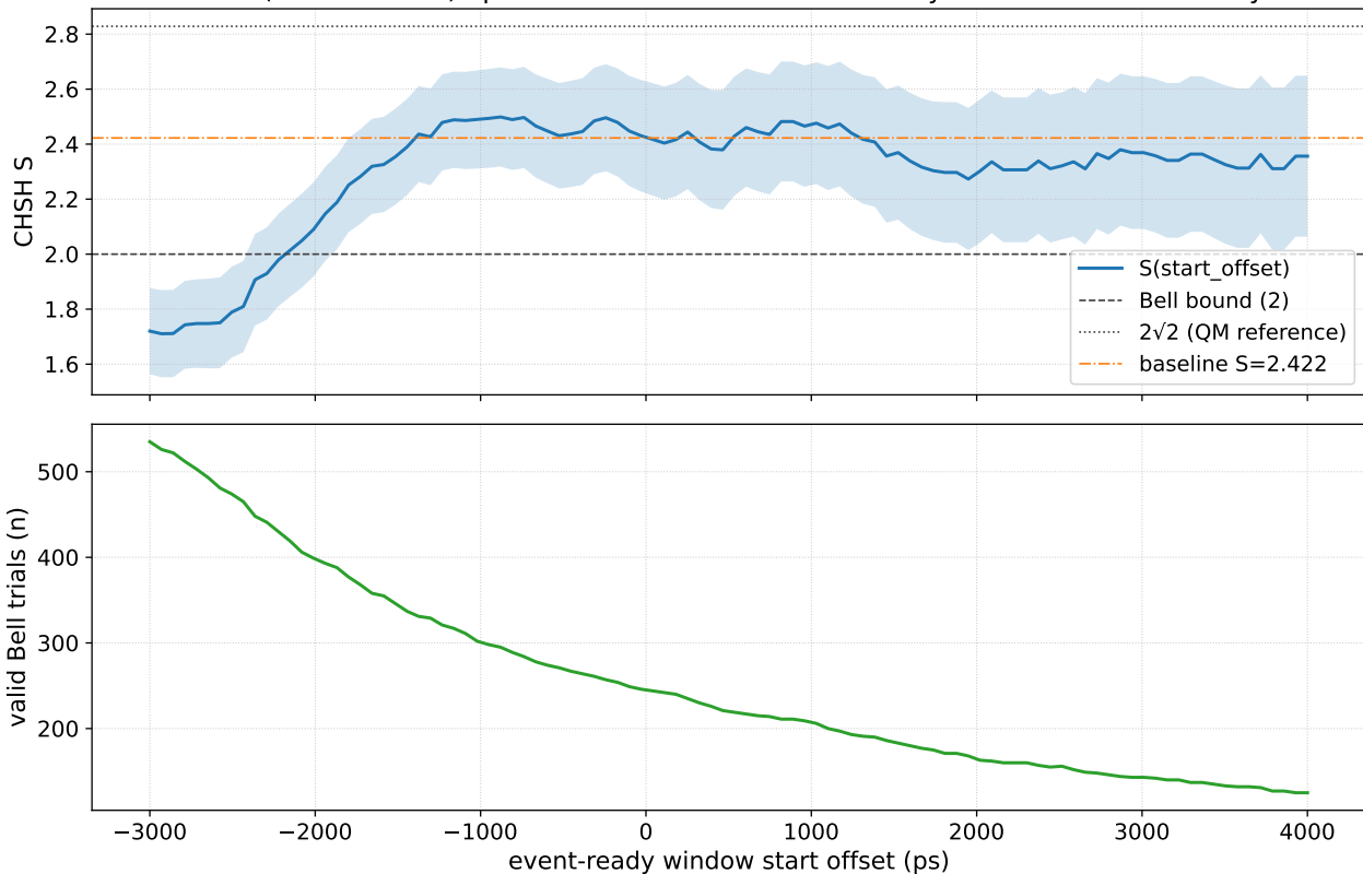
Delft (Hensen 2015) open data: CHSH S and event-ready window start sensitivity
