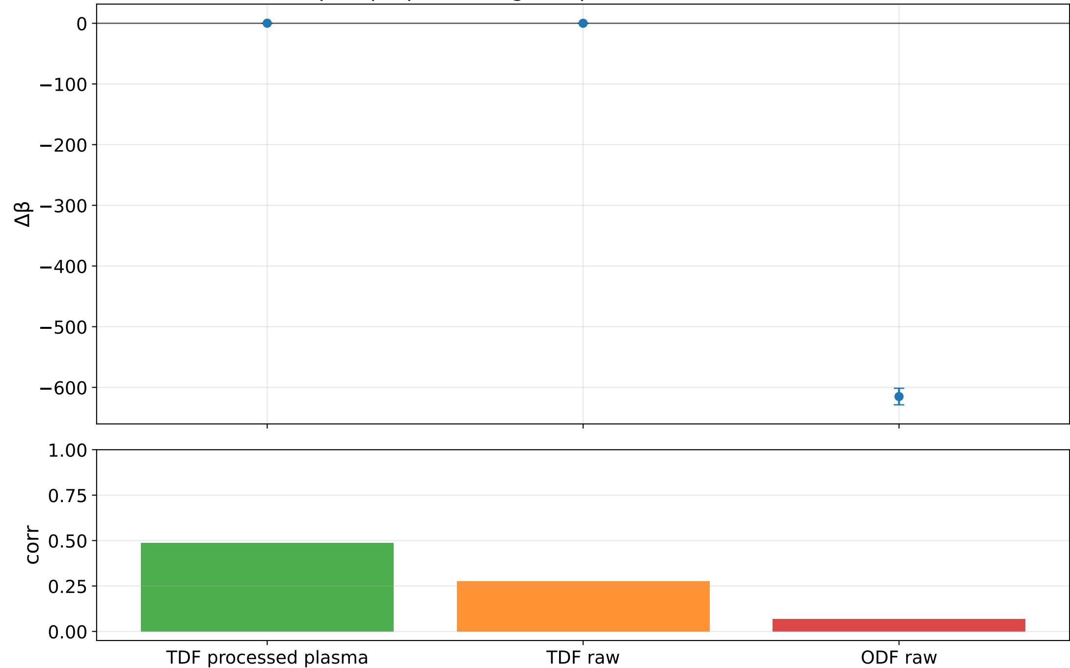
Cassini direct \beta -fit preprocessing comparison (same window, same formula)
