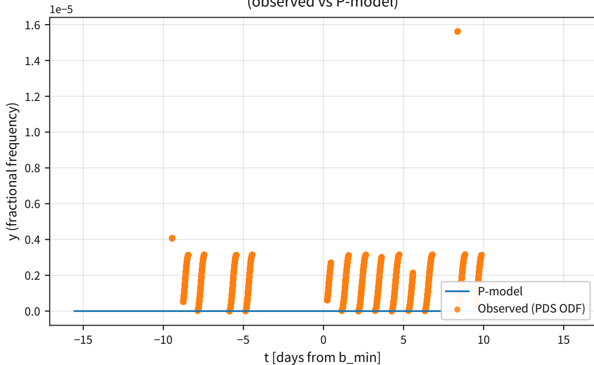
Cassini: Doppler y (observed vs P-model)
