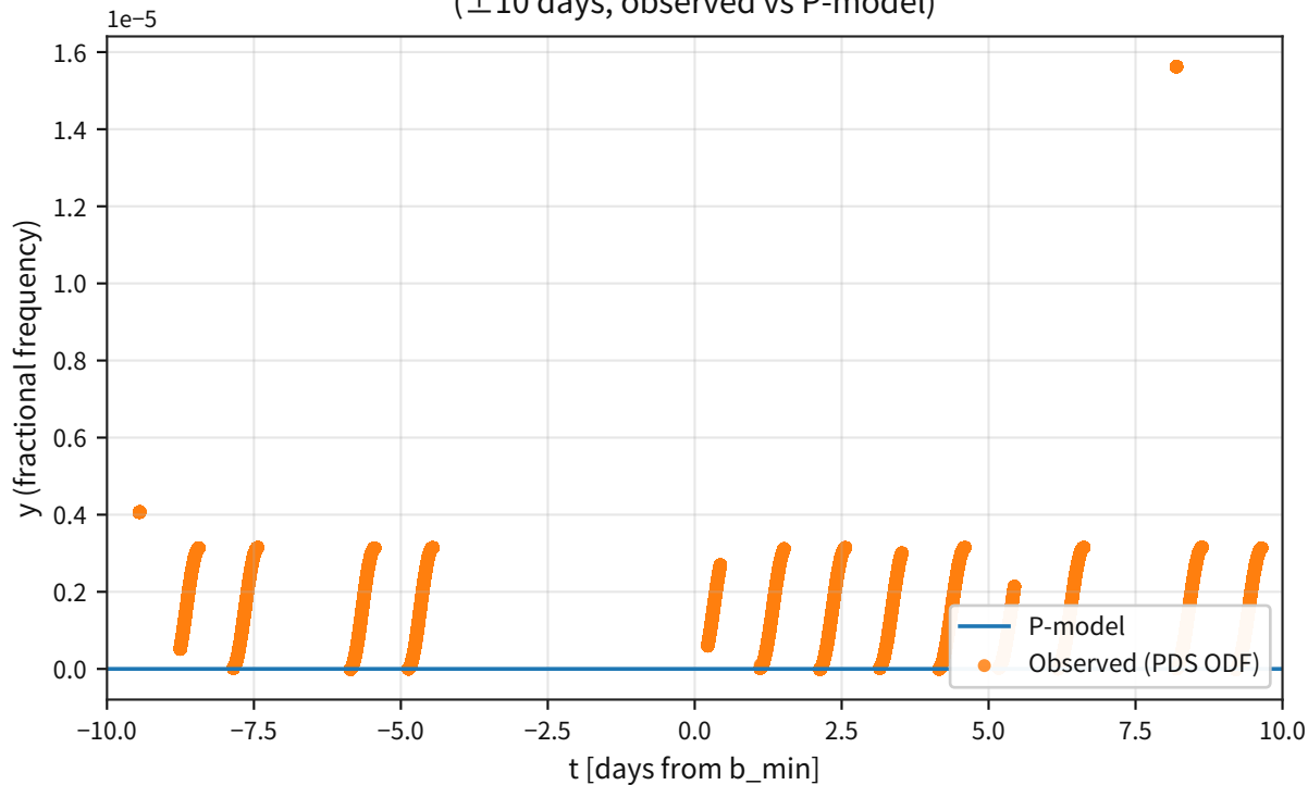
Cassini: Doppler y ( \pm 10 days, observed vs P-model)
