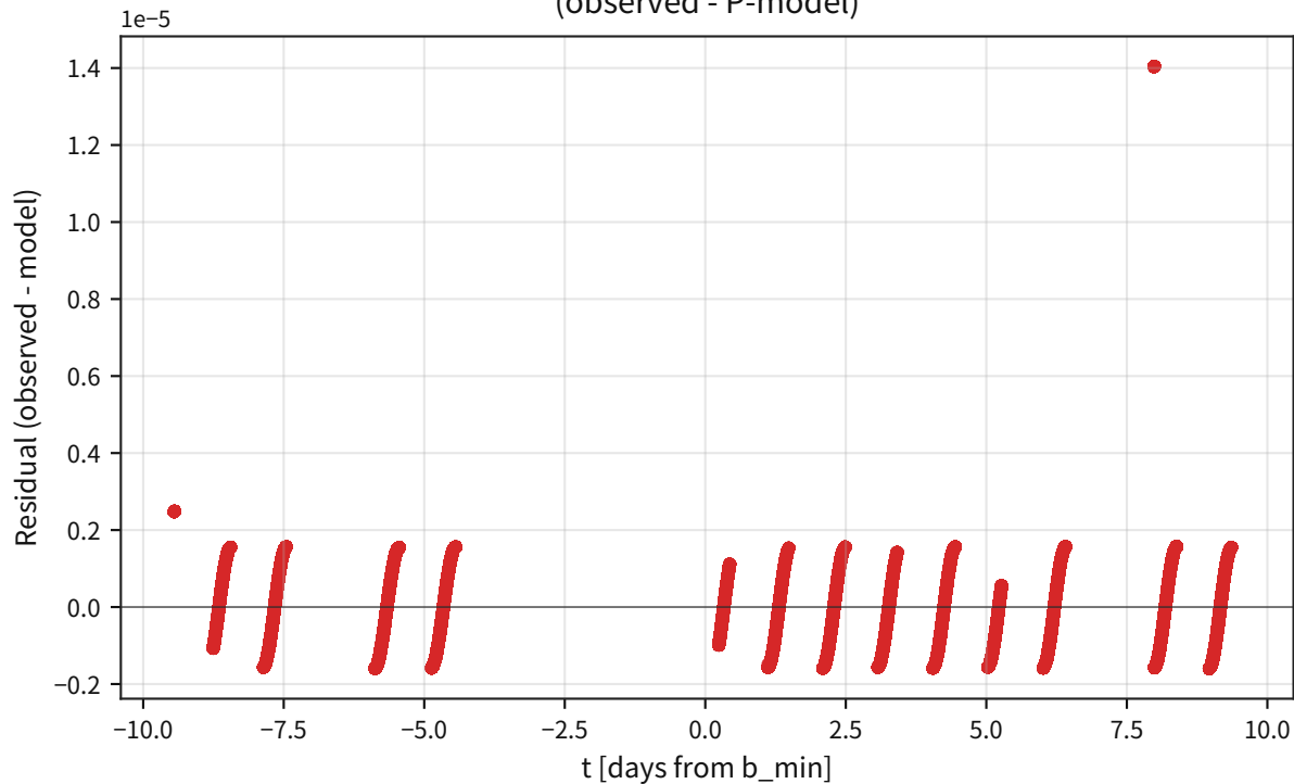
Cassini: residuals (observed - P-model)
