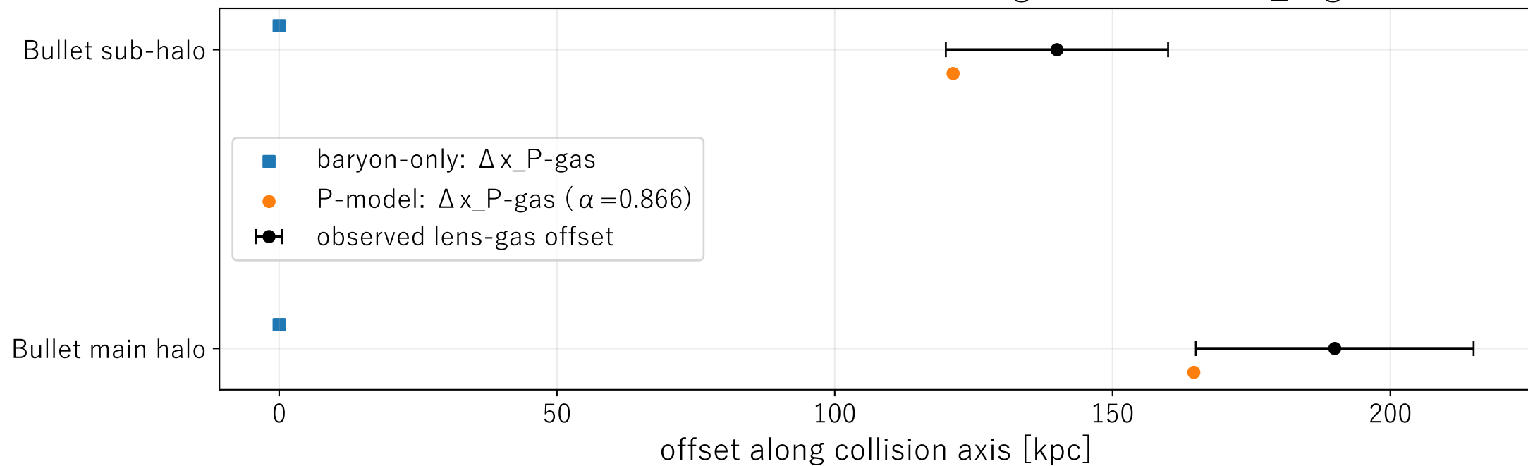
Bullet-cluster offset audit: observed lens-gas vs model \Delta x_{\text{P-gas}}
