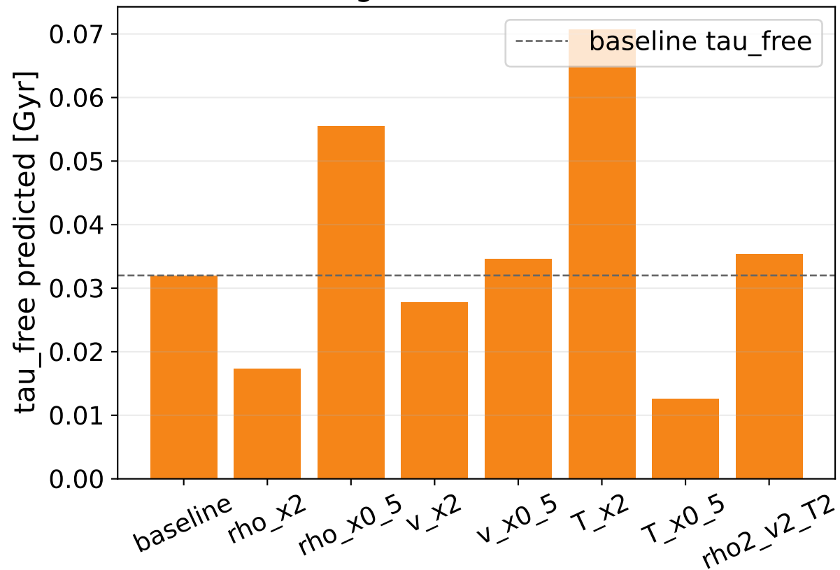
Coarse-grained relaxation time
