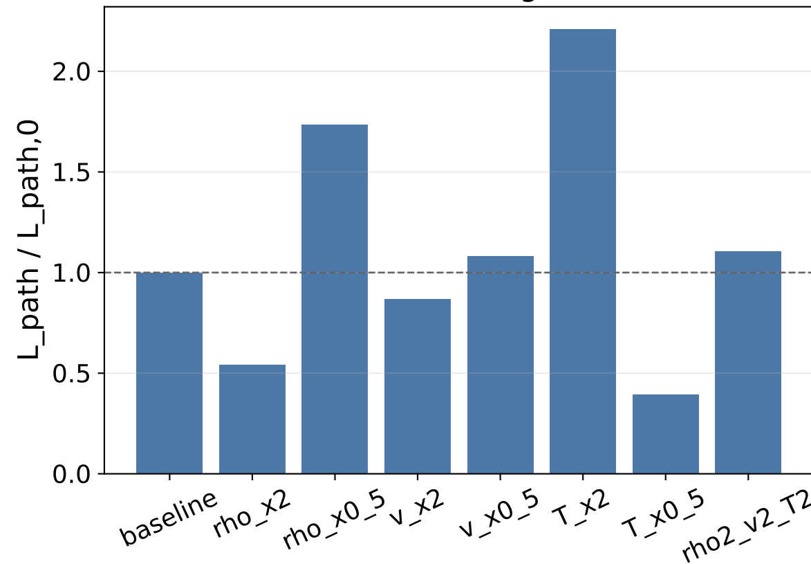
universal scaling ratios
