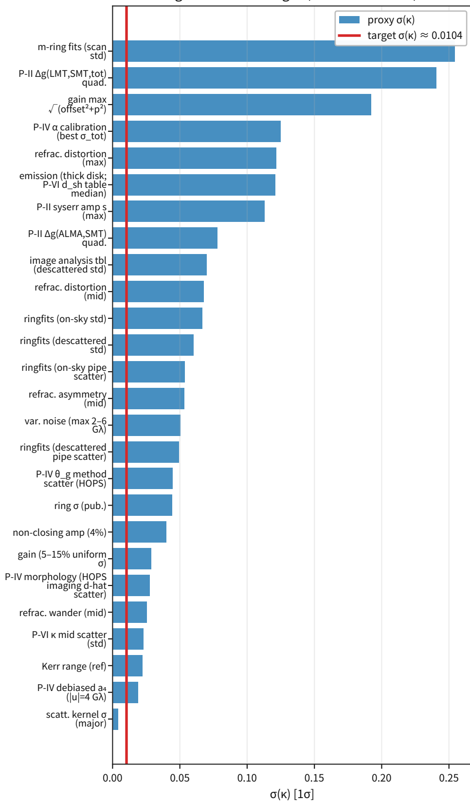
Sgr A* \kappa error budget (scale indicators)
