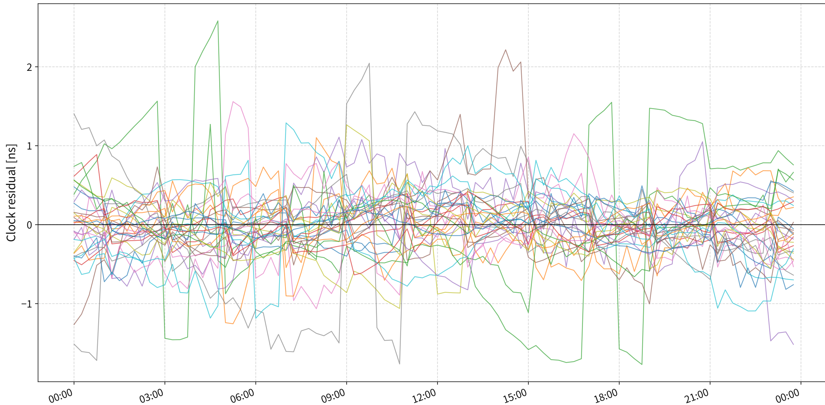
GPS broadcast-clock residuals (BRDC - IGS, all satellites)
