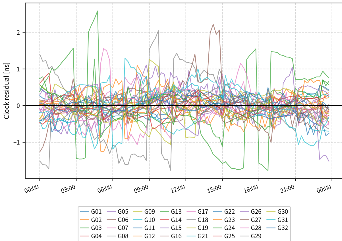
GPS broadcast-clock residuals (BRDC - IGS, all satellites)
