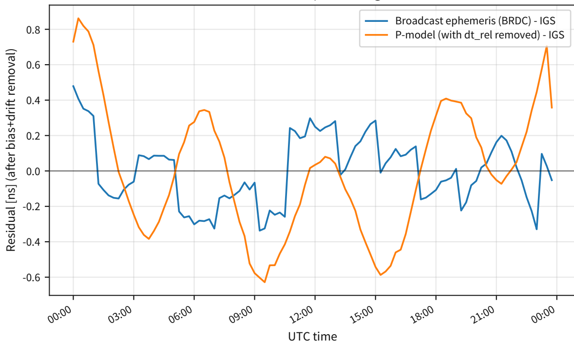
GPS clock residuals: G01 (comparison against observed IGS)
