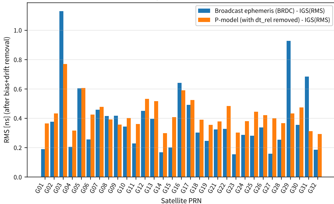
GPS: residual RMS against observed IGS (all satellites)
