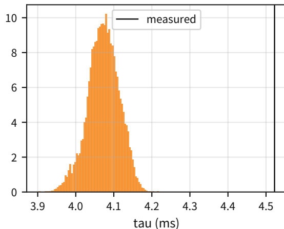
Final spin z_{1d}=0.52
