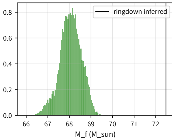
Final mass (det) z_{1d}=0.57
